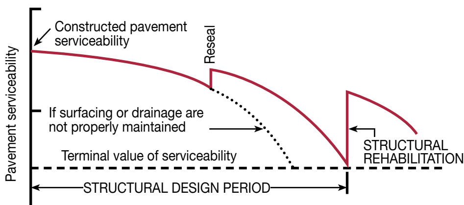
Figure 3-2: Structural design period
