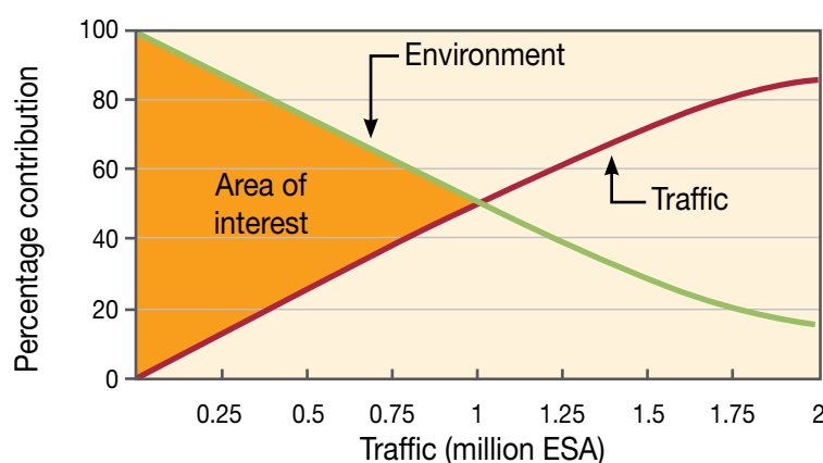
Figure 1-1: Traffic loading versus dominant mechanism of pavement distress (Schematic only)
