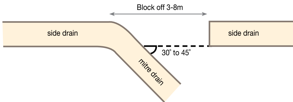
Figure 8-7: Mitre drain angle greater than 45 degrees
