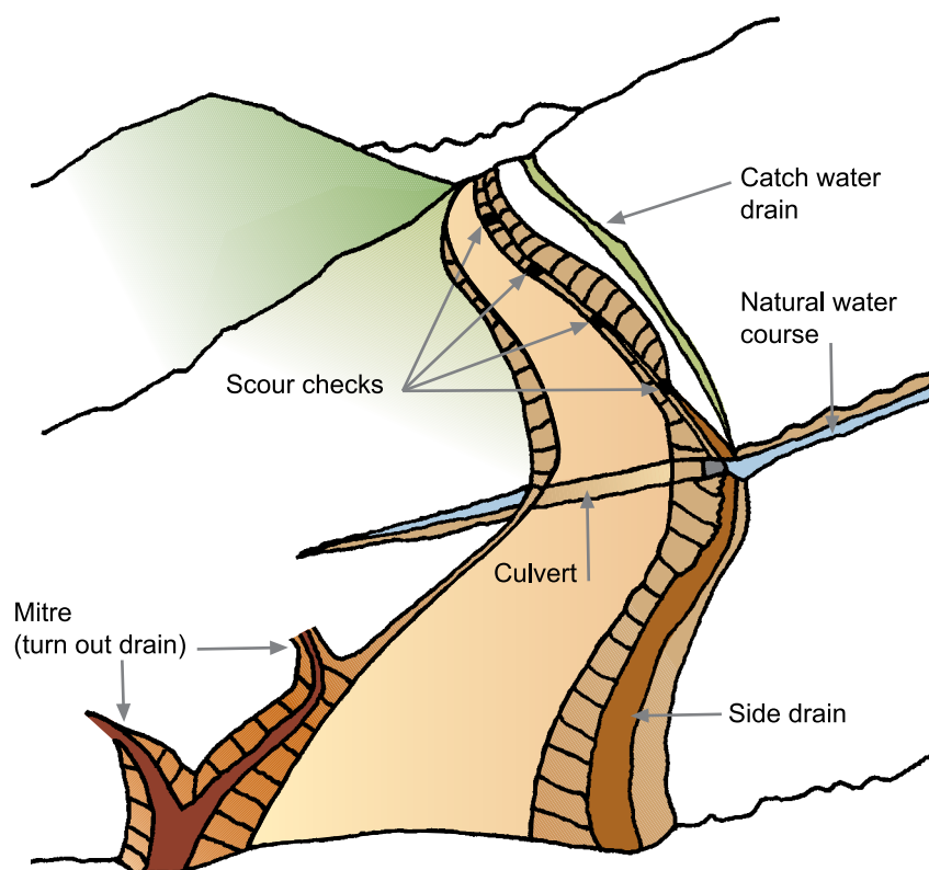
Figure 2-3: Drainage elements
