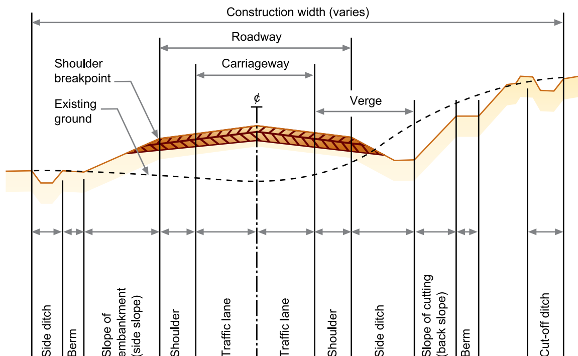
Figure 2-2: Cross section
