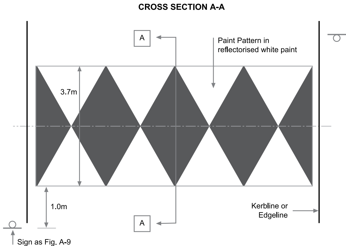
Figure 4A-5: Village treatment – Watts profile hump
