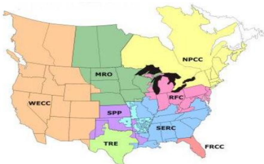
Figure 2: NERC regions
