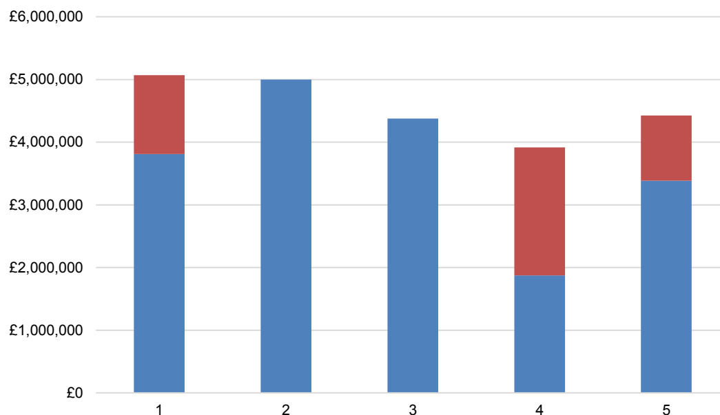
Figure 3: Capital costs of new nuclear power stations (per MW capacity)
