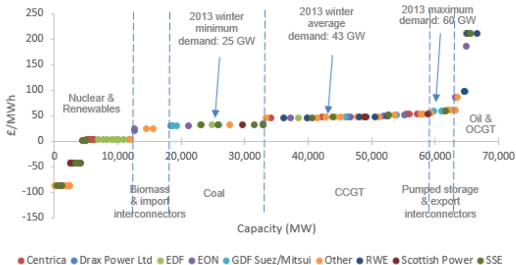
Figure 2: Merit order of GB generators (31/10/13)
