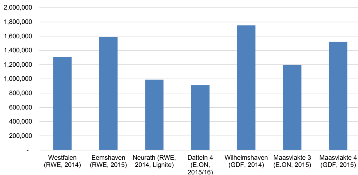
Figure 2: Capital costs of new (non-CCS) coal-fired power stations (per MW capacity)
