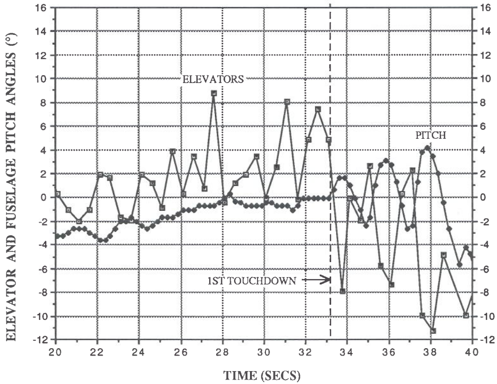
FIG 1: ACCIDENT LANDING ELEVATOR AND PITCH ANGLES
