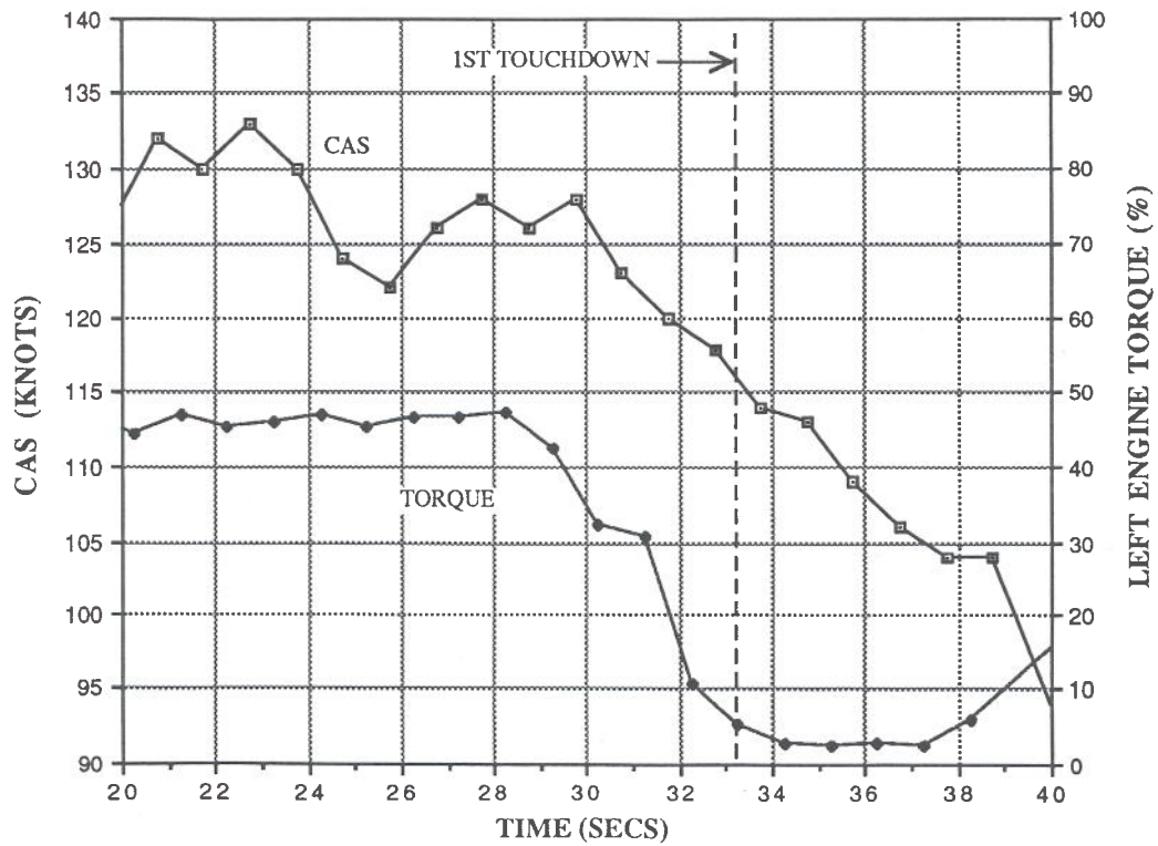
FIG 2: ACCIDENT LANDING AIRSPEED AND POWER
