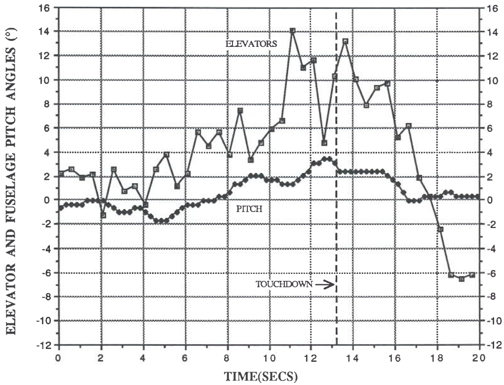
FIG3: PREVIOUS LANDING ELEVATOR AND PITCH ANGLES
