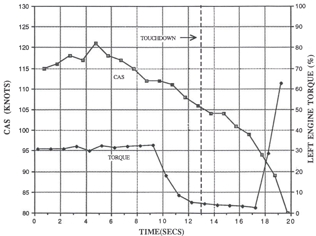
FIG 4: PREVIOUS LANDING AIRSPEED AND POWER
