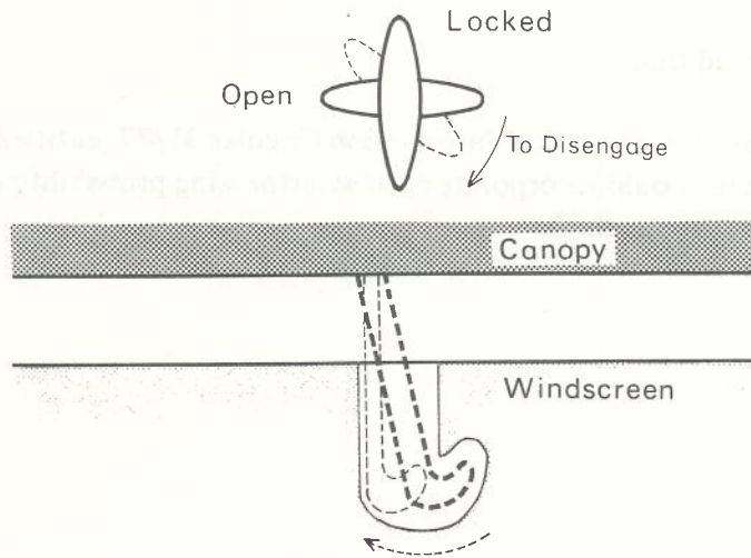
CANOPY LOCKING ACTION - VIEWED FROM ABOVE
