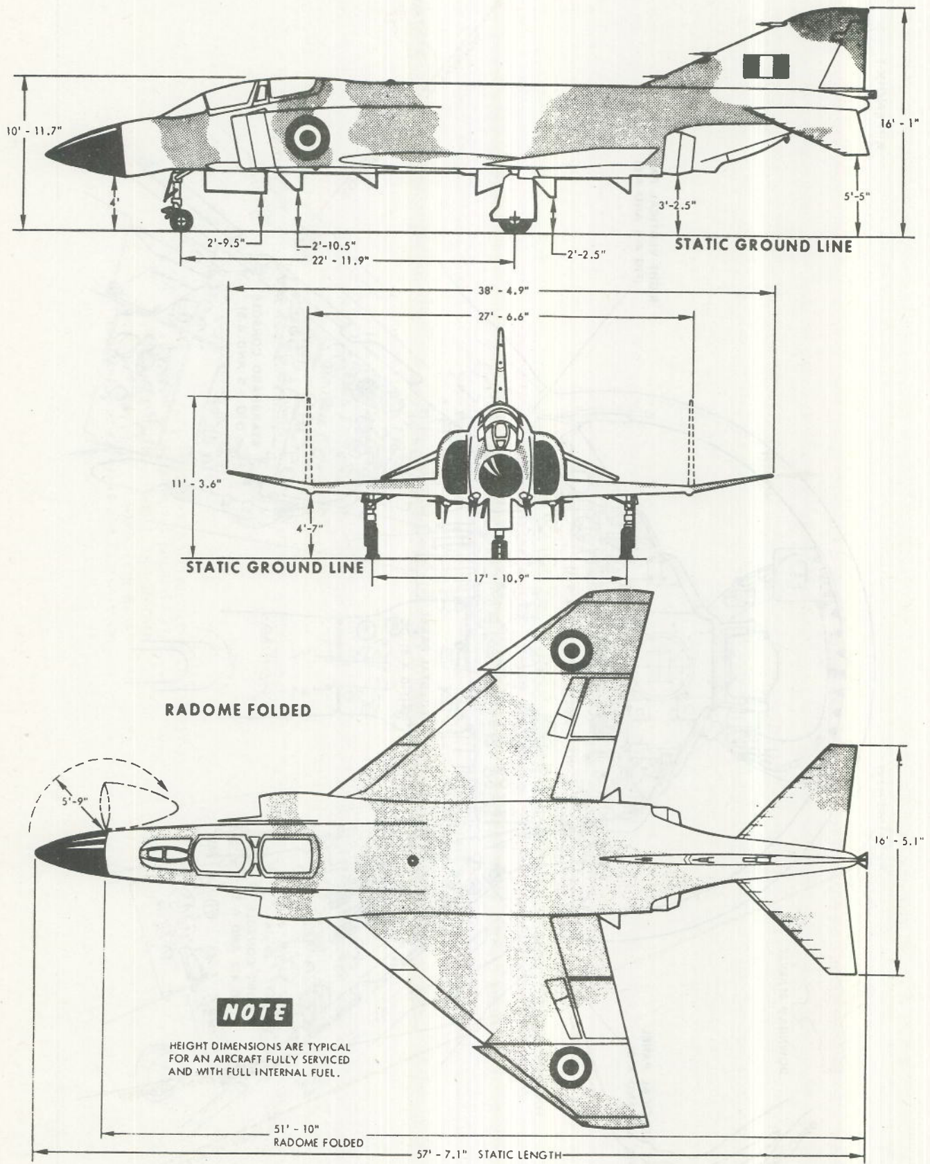
Figure 3-3. Principal Dimensions
