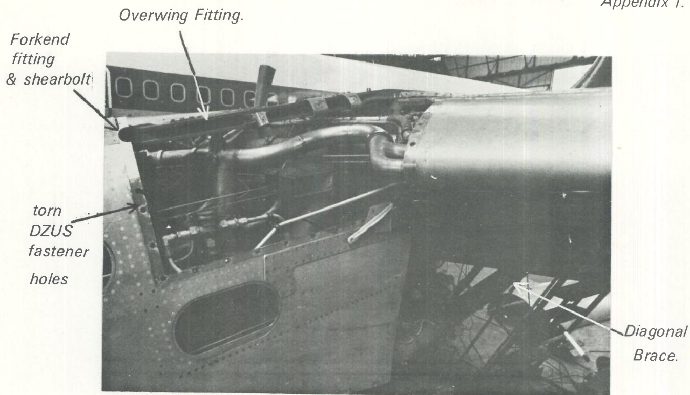
General View of Wing/Pylon Junction ( No 2 Pylon )
