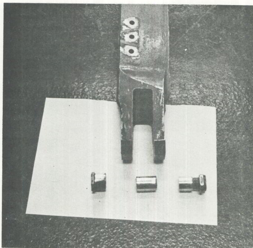
No 2 Pylon Overwing Fitting Fork End and Shear Bolt as removed from G-APFH.
