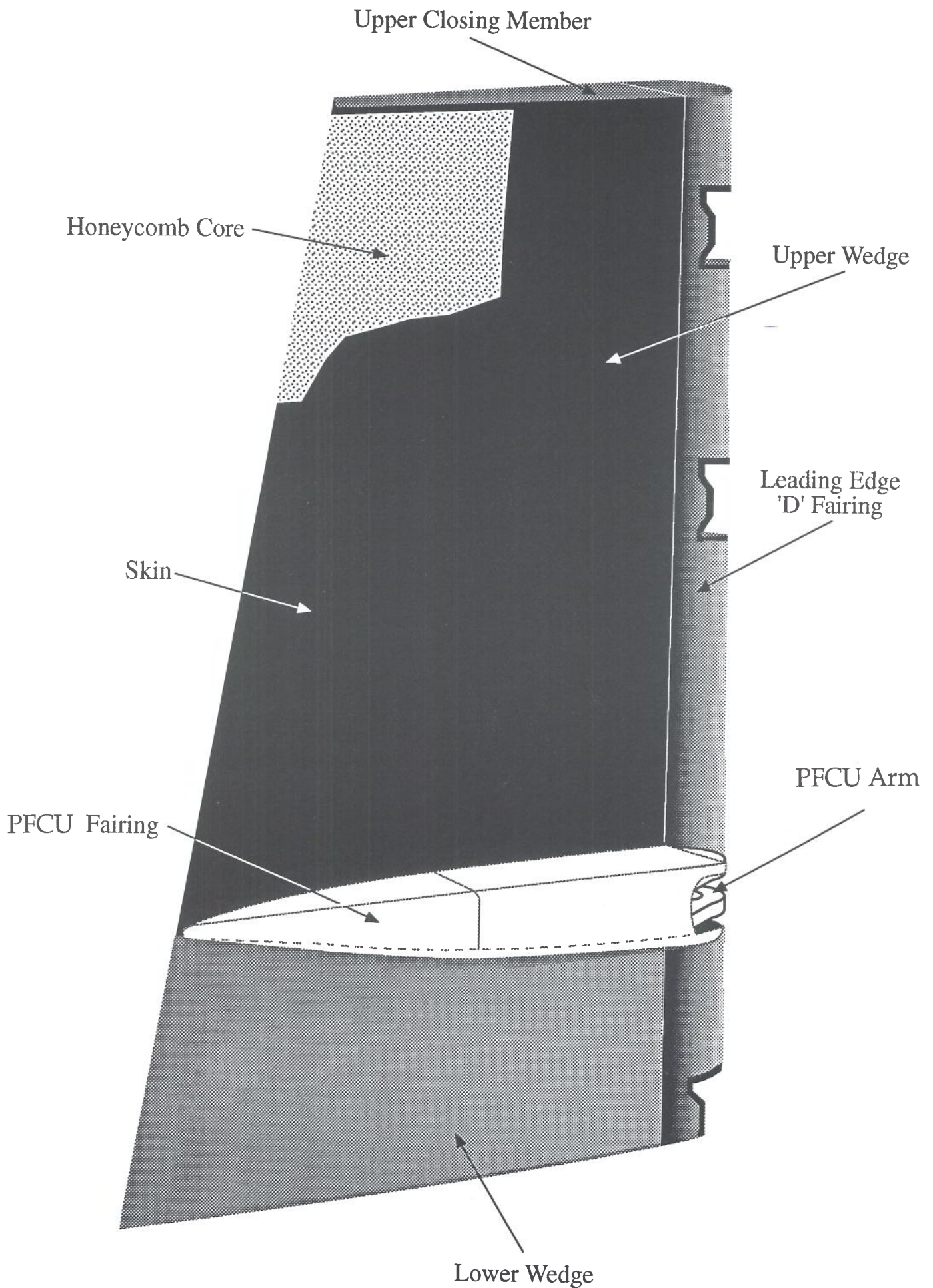
Upper Rudder Showing Construction Features
