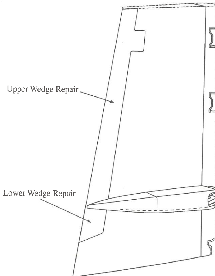
Details of Upper Rudder Repair Scheme
