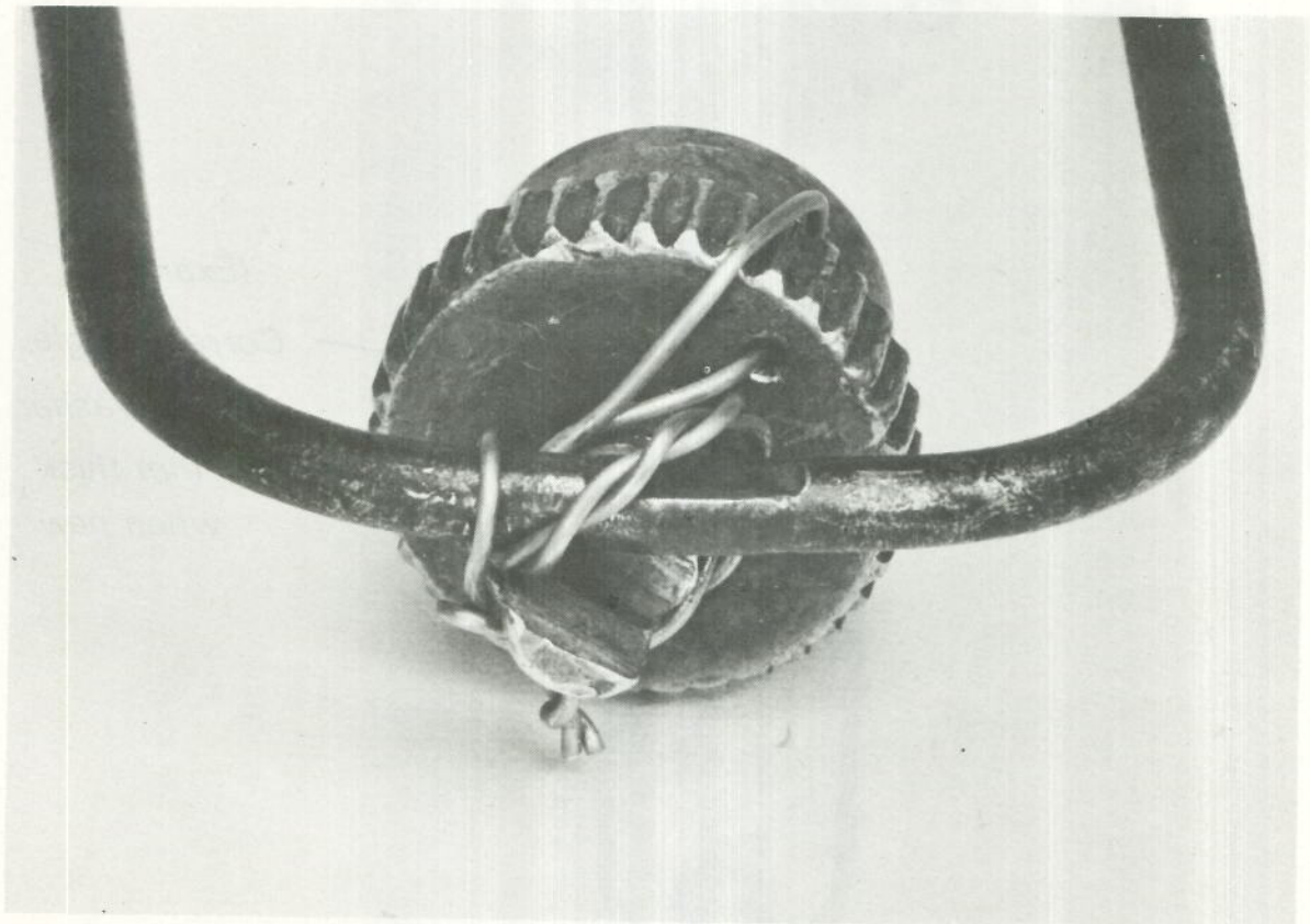
Showing fractured anchorage lug and incorrect routing of locking wire
