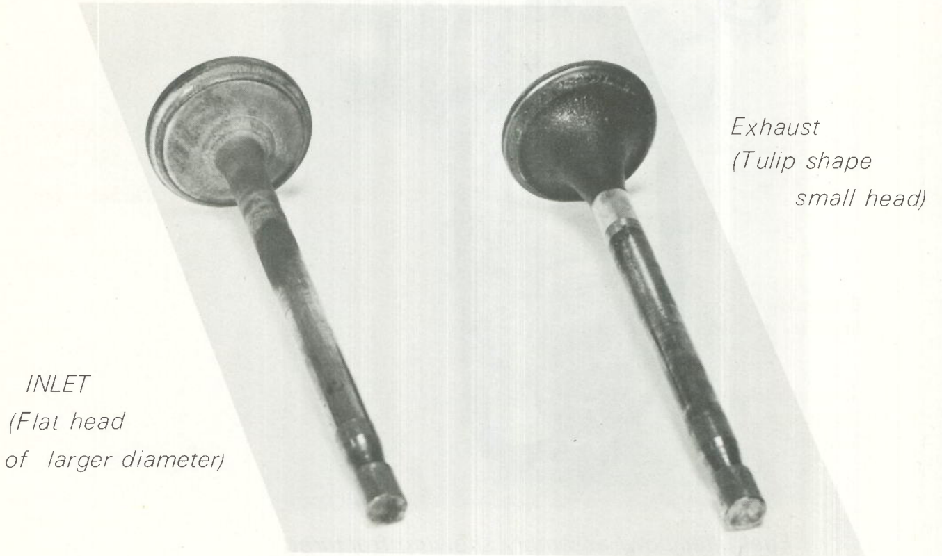
Showing differences in heads of valves
