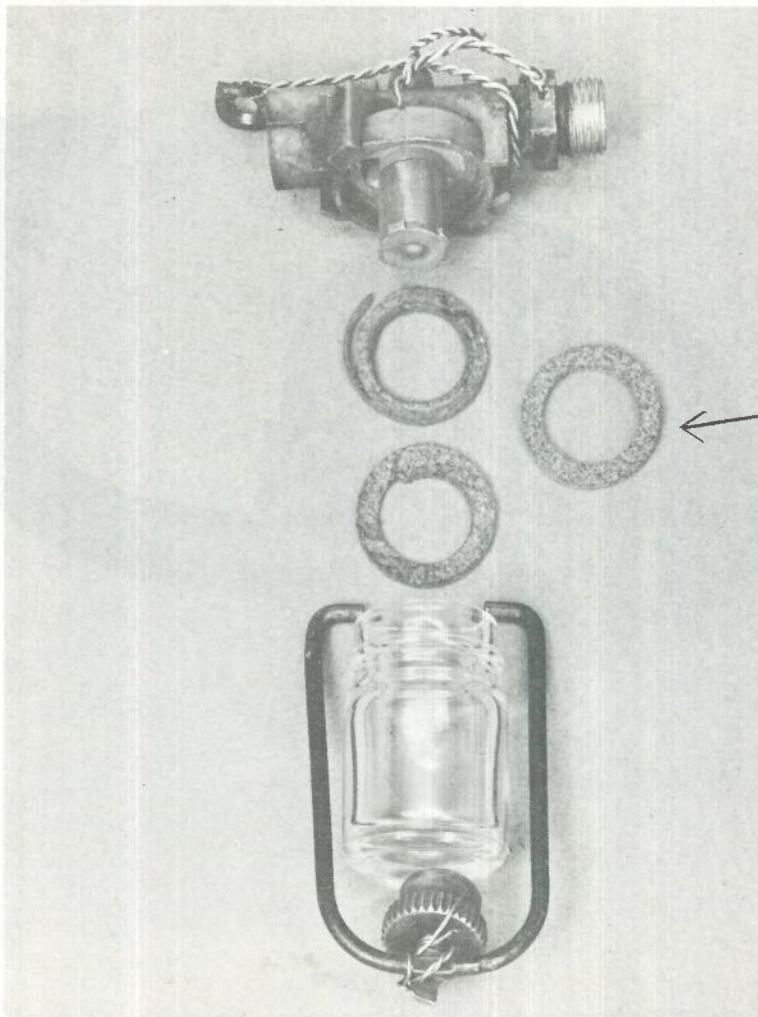
Disassembled filter bowl showing two thin and damaged cork sealing washers
