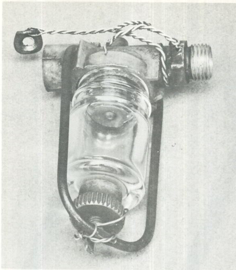
Fuel filter bowl assembly showing fractured anchorage lug and incorrect wire locking
