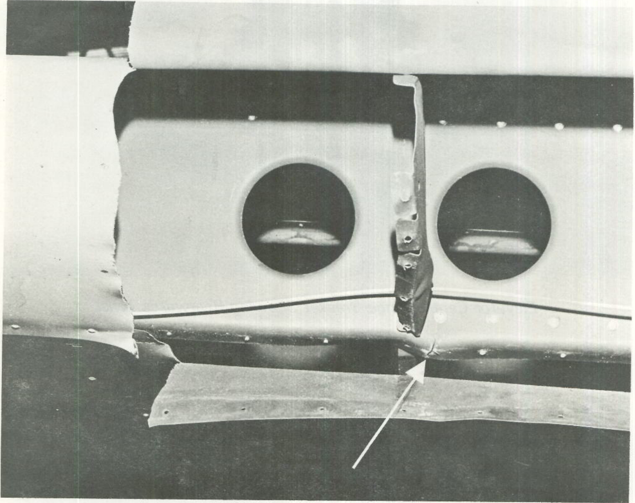
Right Hand Wing Lower Spar Showing Compression Buckle And Fracture
