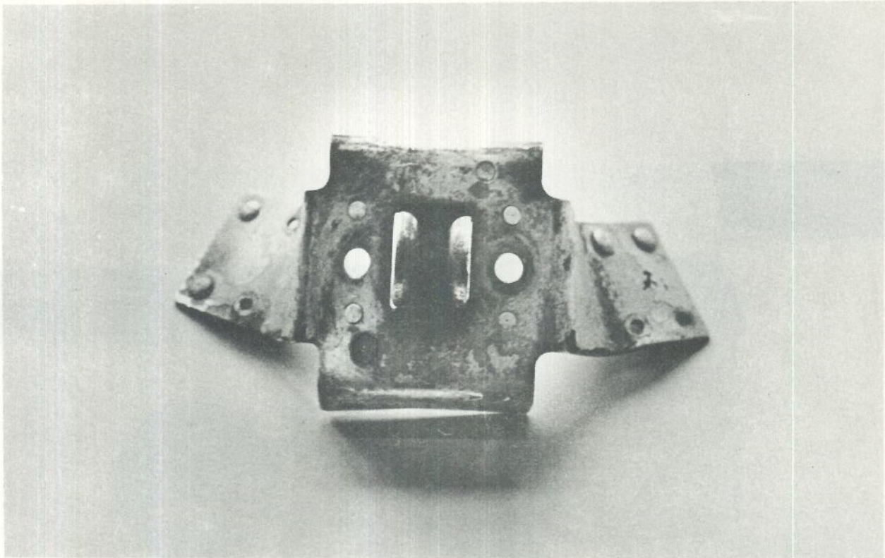
Elevator Centre Hinge Bracket Showing Rearwards Twist And Elongation Of Bolt Holes.
