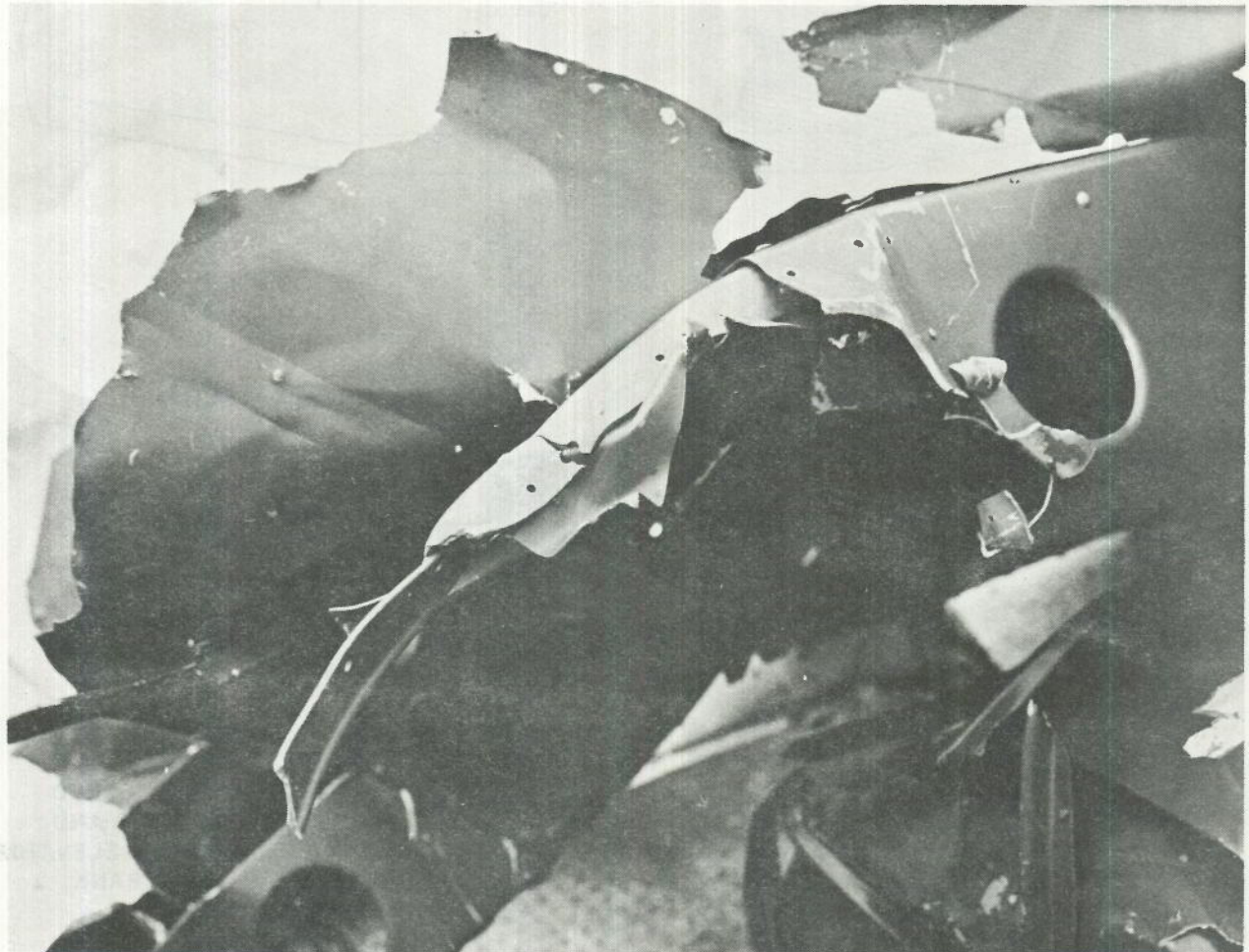
Left Wing Showing Compression Collapse Of Spar (Download)
