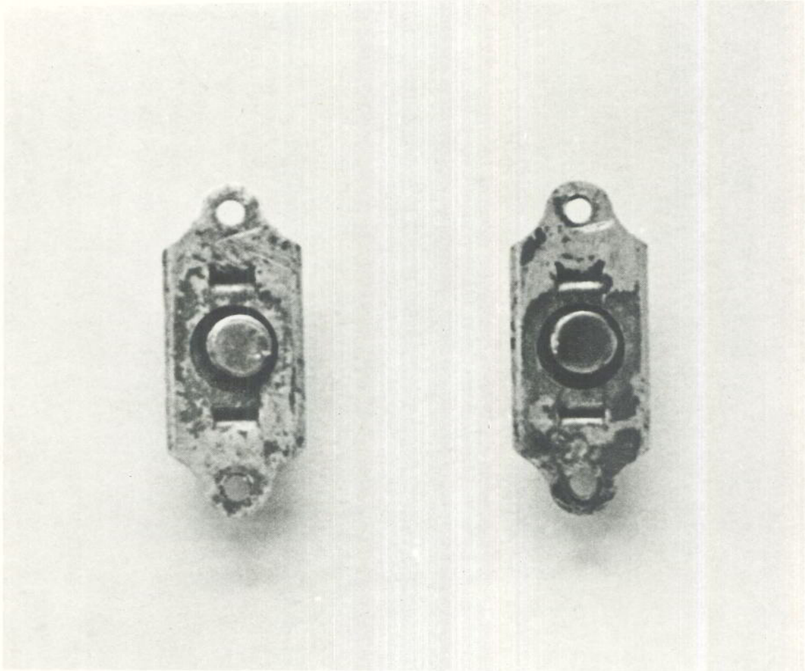
Showing Sheared Bolts Tail-Fin Attachments.
