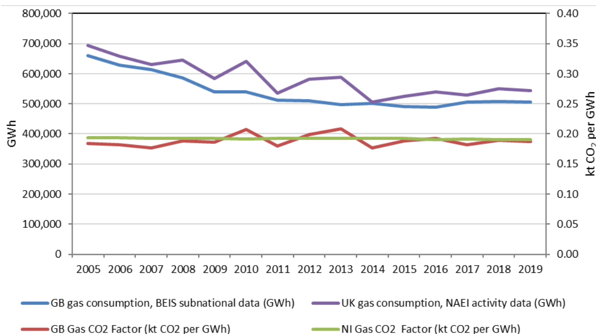
Figure 2 Natural Gas consumption and emission factors, weather-corrected and non-weather-corrected
