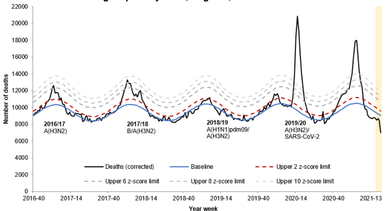
Figure 1: Weekly observed and expected number of all-cause deaths in all ages, with the dominant circulating respiratory virus, England, 2016 to week 20 2021
