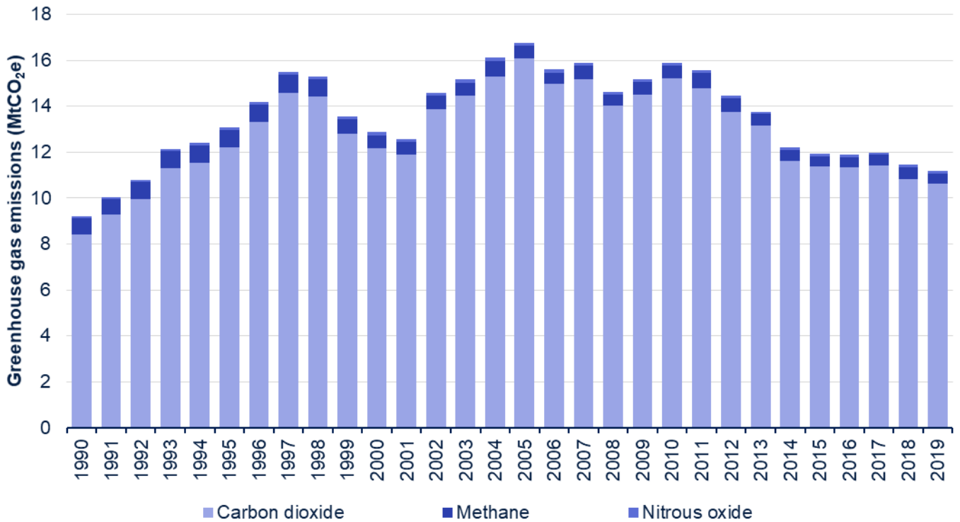
Figure 10: Greenhouse gas end user emissions from the exports sector, UK, 1990-2019 (MtCO 2e )
