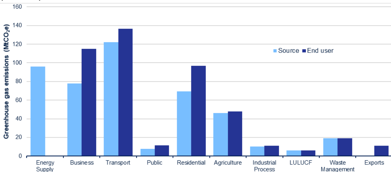
Figure 1: Greenhouse gas emissions by source sectors and end user sectors, UK 2019 (MtCO 2e )
