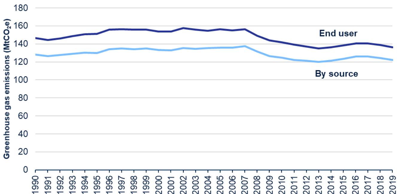
Figure 4: Greenhouse gas end user emissions from transport, UK 1990-2019 (MtCO 2e )
