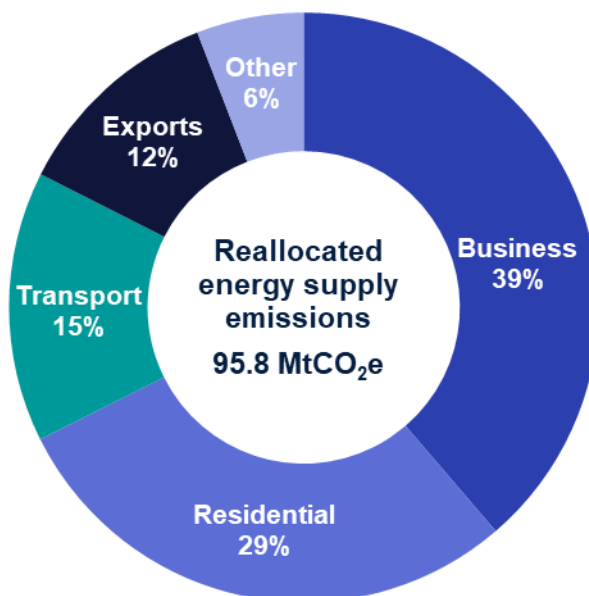
Figure 3: Breakdown of greenhouse gas emissions reallocated from the energy supply sector to the end user sectors, UK 2019
