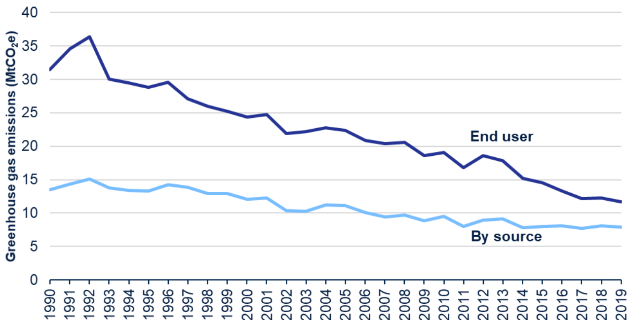
Figure 9: Greenhouse gas end user emissions from the public sector, UK, 1990-2019 (MtCO 2 e)
