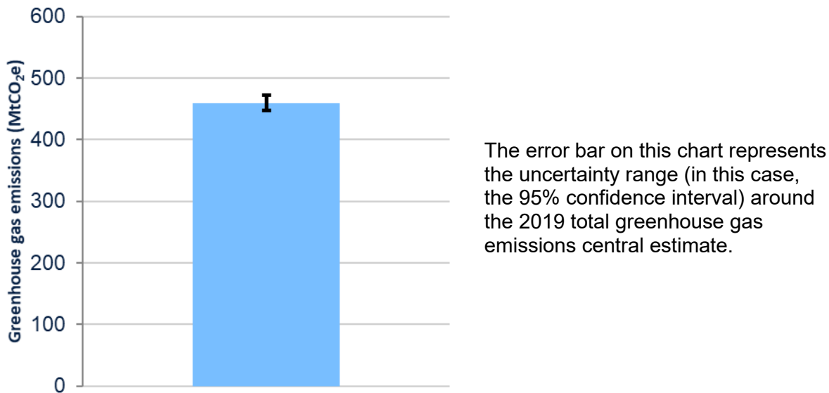
Figure 11: Illustration of uncertainty in estimates of UK Greenhouse Gas emissions, UK, Crown Dependencies and Overseas Territories, 2019 (MtCO 2 e)
