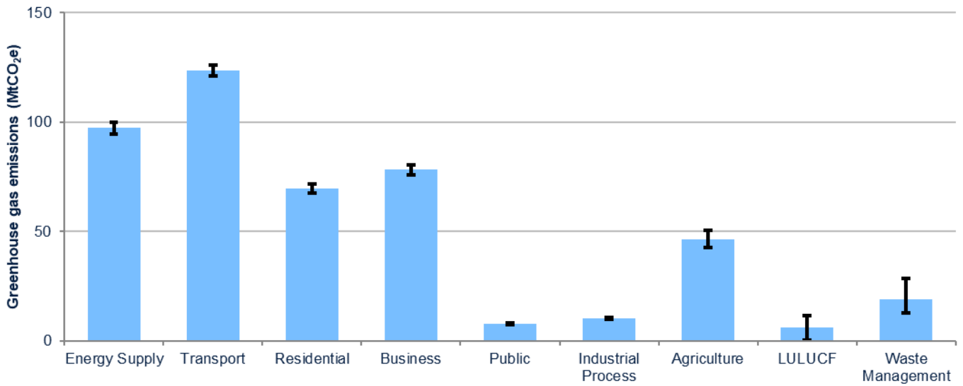
Figure 13: Illustration of uncertainty in estimates of UK Greenhouse Gas emissions by sector
