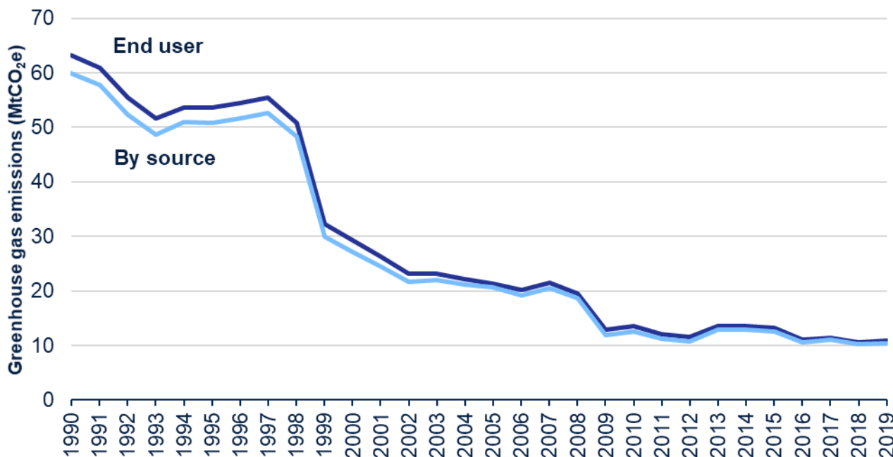
Figure 8: Greenhouse gas end user emissions from industrial processes, UK, 1990-2019 (MtCO 2 e)
