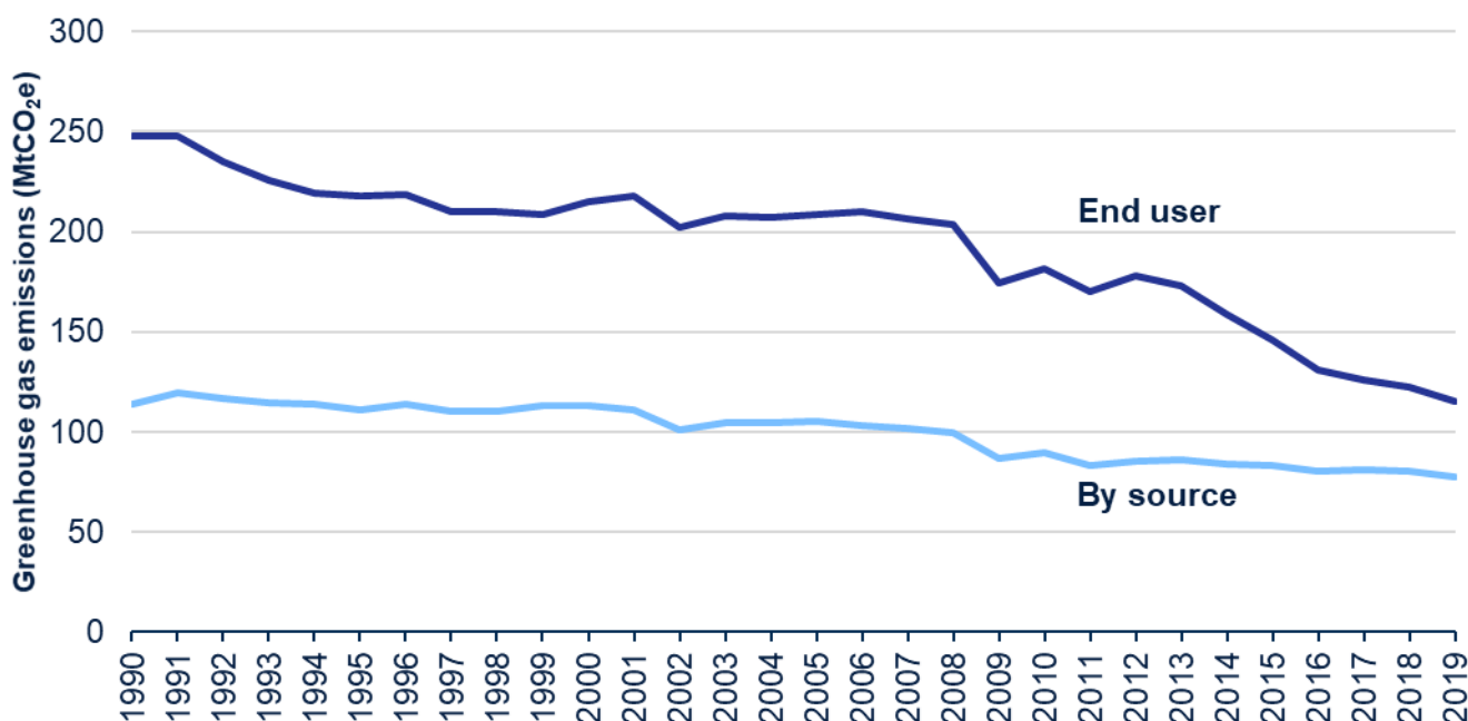
Figure 5: Greenhouse gas end user emissions from business, UK 1990-2019 (MtCO 2e )
