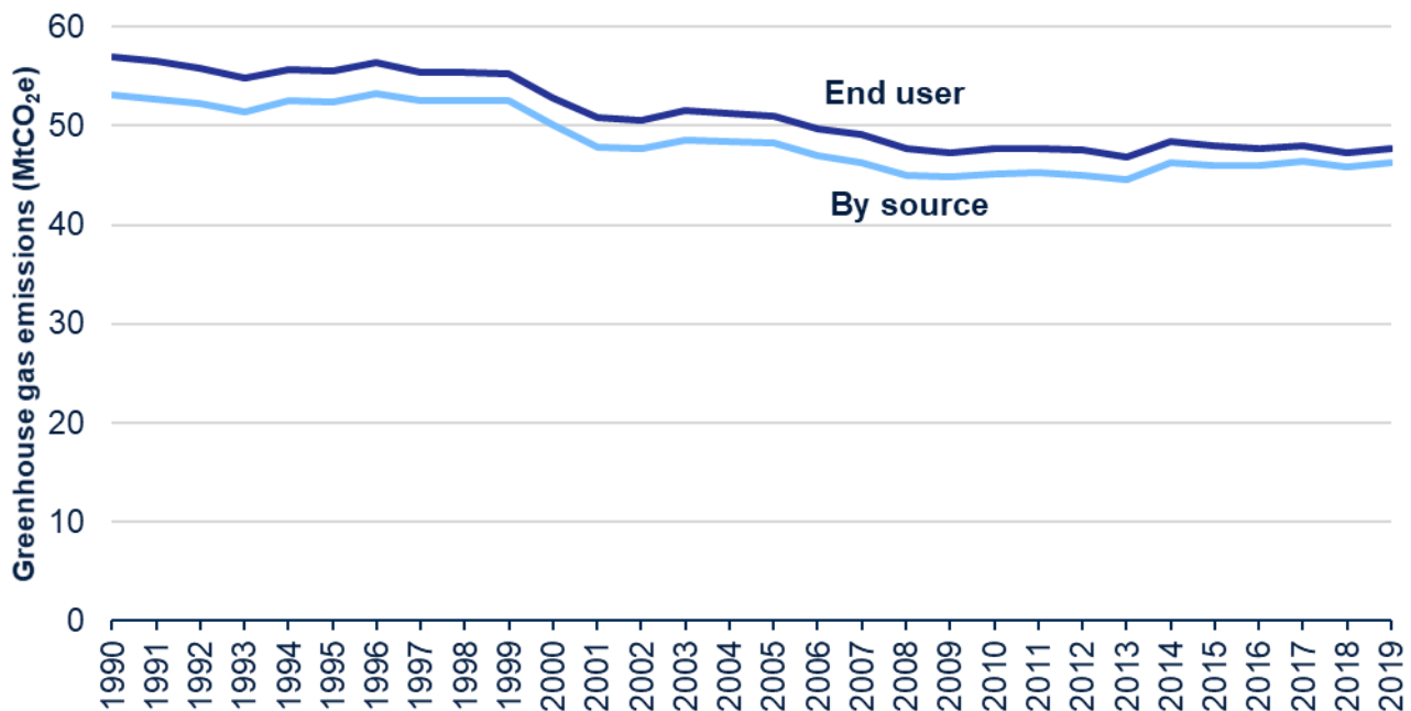
Figure 7: Greenhouse gas end user emissions from agriculture, UK 1990-2019 (MtCO 2 e)
