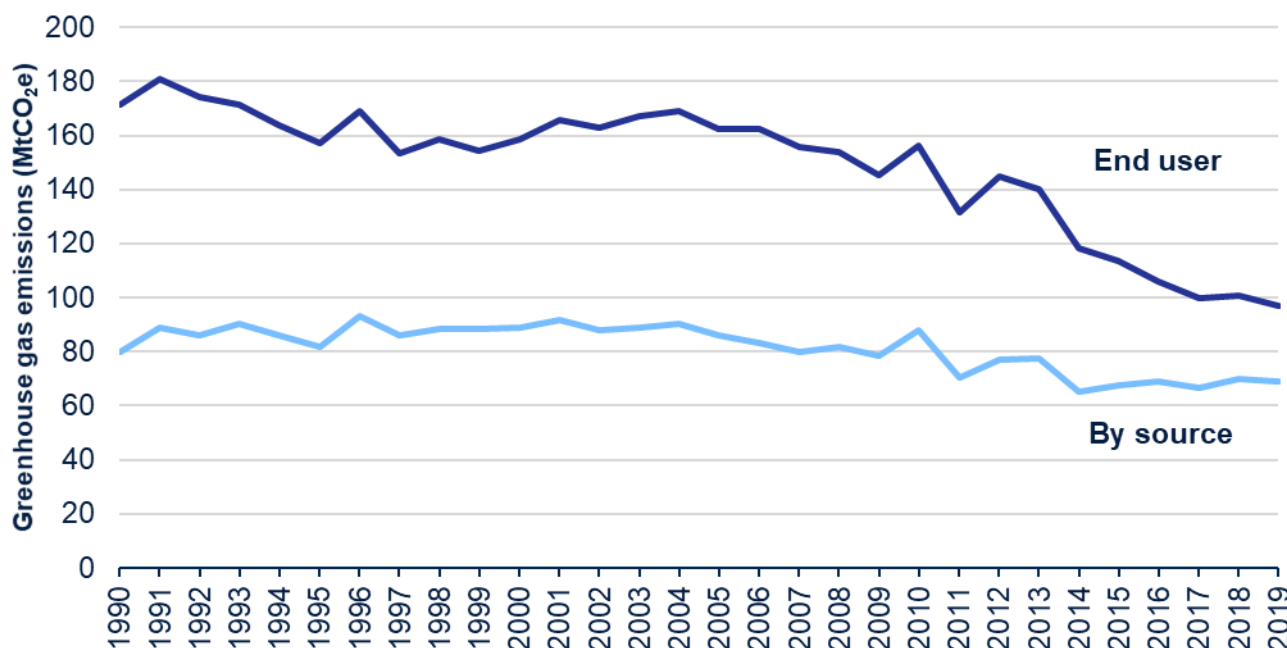
Figure 6: Greenhouse gas end user emissions from the residential sector, UK 1990-2019 (MtCO 2 e)
