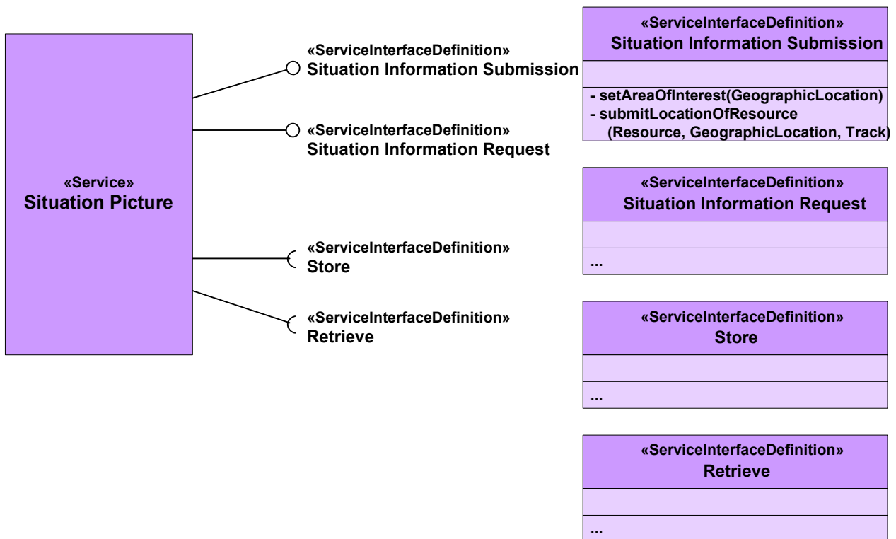
SOV-2 UML Representation
