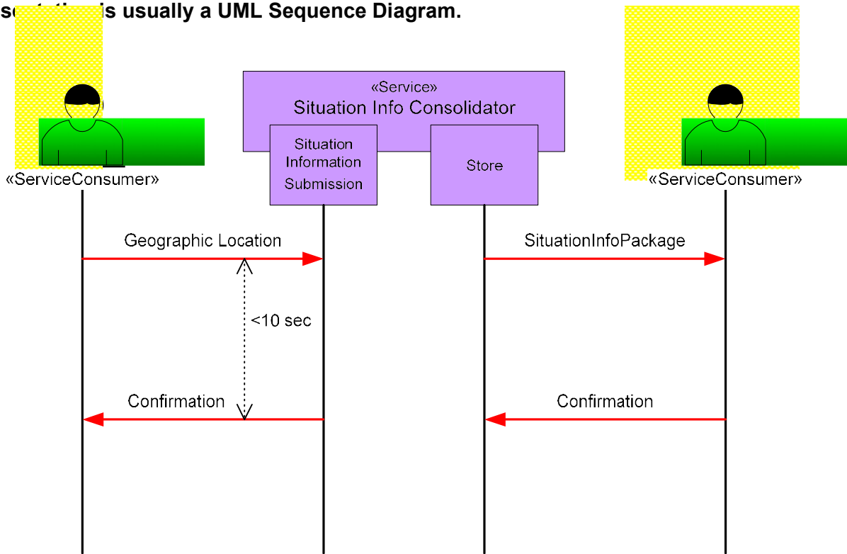
SOV-4c Sequence Diagram representation
