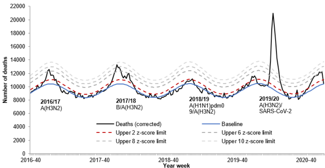
Figure 1: Weekly observed and expected number of all-cause deaths in all ages, with the dominant circulating respiratory virus, England, 2016 to week 53 2020
