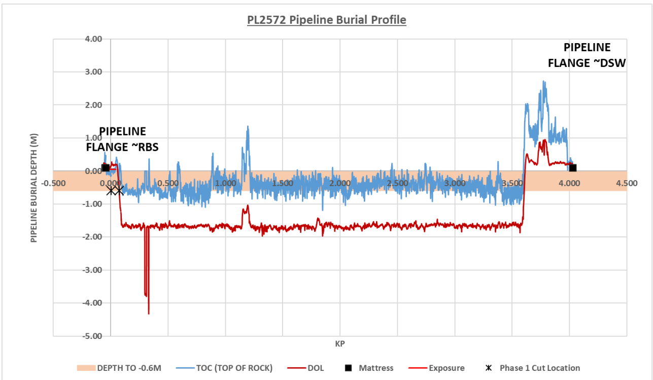
Figure 3.3.2: PL2572 depth of burial profile
