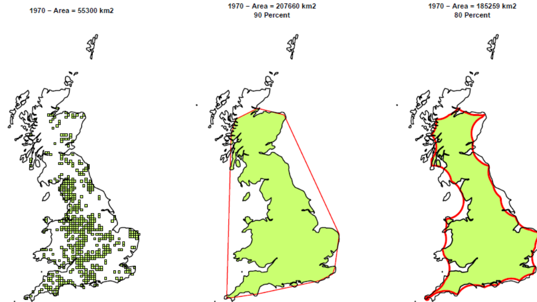
Figure 1. Example area of extent maps for Elodea canadensis using data from the 1970-1979 time period. The first map shows the 10km occurrence data, the second map shows the Minimum Convex Polygon (outlined by a red line) and its intersection with the land (green filled region) and third map shows the alpha hull (outlined by a red line) and its intersection with the land (green filled region). The labels above each map give the total area of distinct 10km squares, the area of the MCP/GB land intersection and the area of the alpha hull/GB land intersection respectively.
