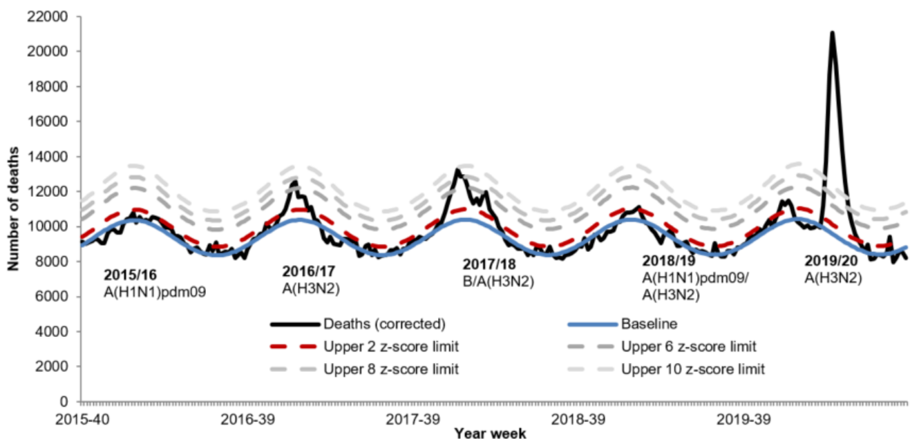
Figure 1: Weekly observed and expected number of all-cause deaths in all ages, with the dominant circulating influenza A subtype, England, 2015 to week 38 2020
