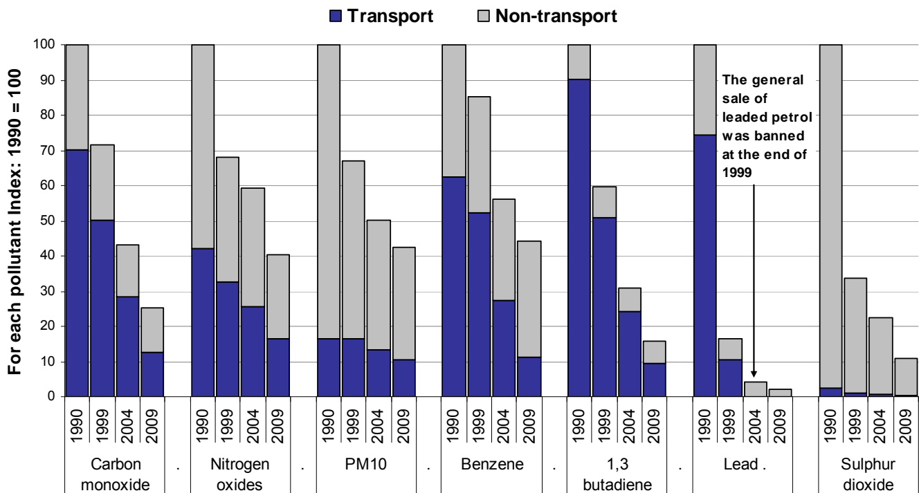
Chart 5 - UK air pollutant emissions: 1990, 1999, 2004 and 2009
