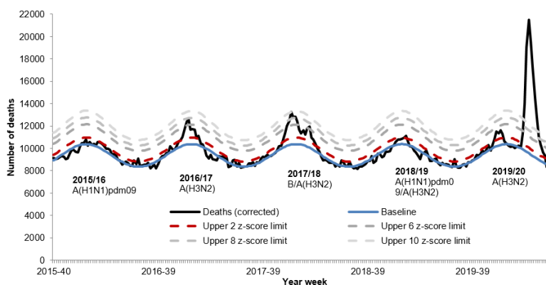
Figure 1: Weekly observed and expected number of all-cause deaths in all ages, with the dominant circulating influenza A subtype, England, 2015 to week 24 2020
