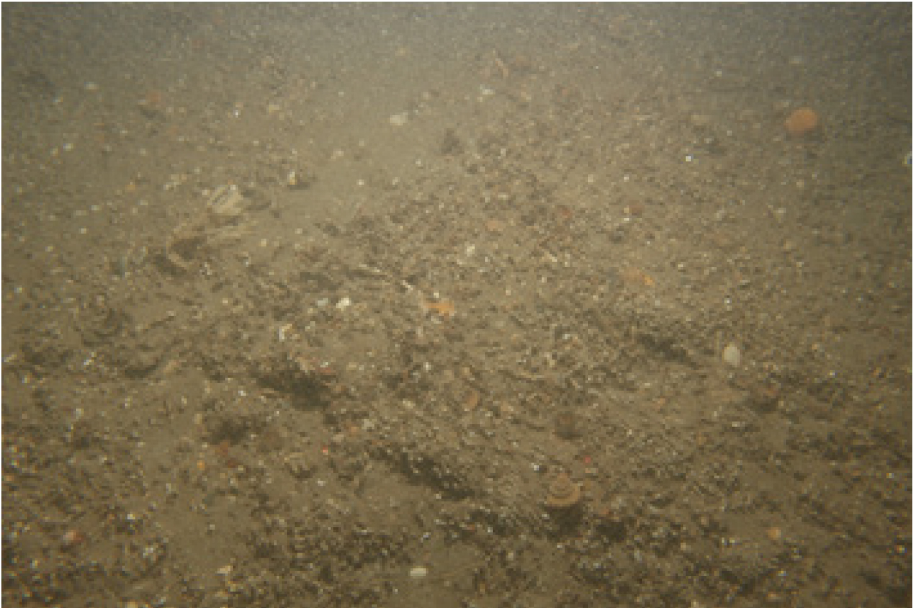
Subtidal coarse sediment © JNCC/CEFAS
