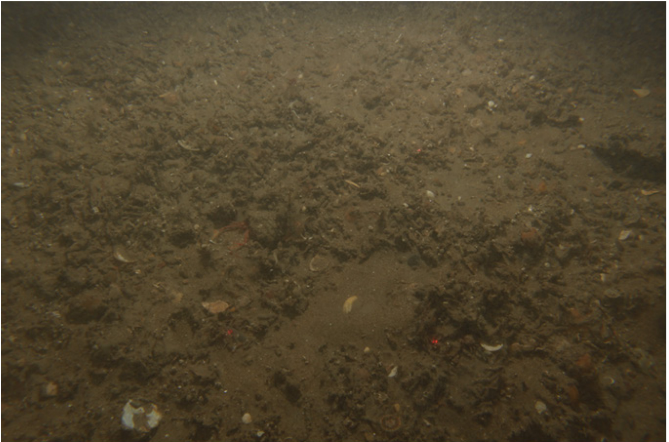
Subtidal mixed sediments © JNCC / Cefas
