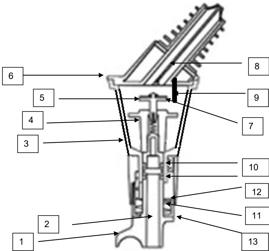
Figure 2 25 ml measure – Sectional general assembly
