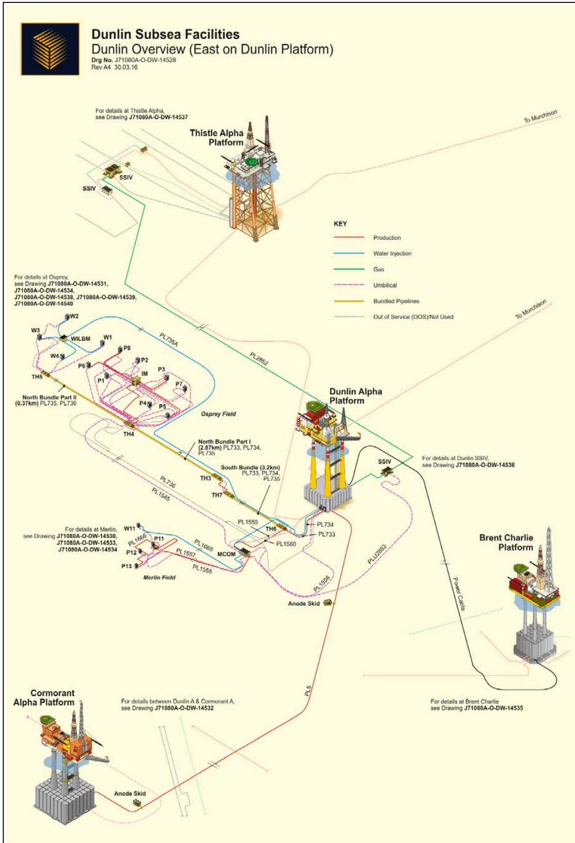
Figure 1-3: Greater Dunlin Area Field Layout
