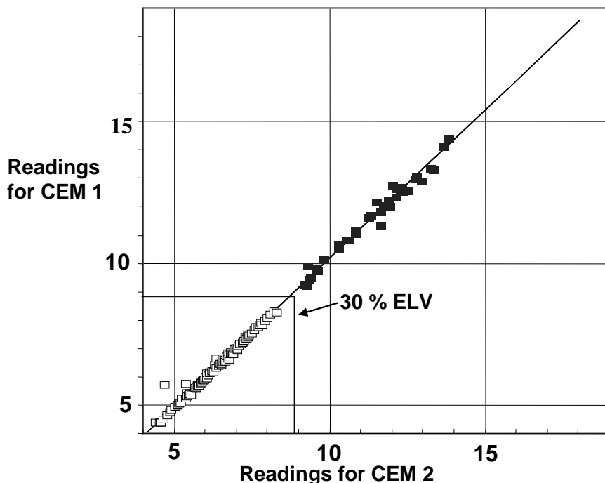
Figure 2 — Graphical representation of measured signals used for determination of reproducibility under field conditions
