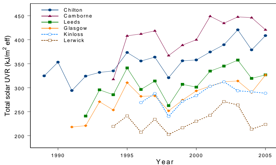
Figure 9: Total yearly erythemal \text{UVR}_{\text{eff}} data for the six UK sites. Chilton (1989- 2005), Glasgow (1991– 2005), Leeds (1992–2005), Camborne (1994-2005), Lerwick (1994-2005) and Kinloss (1996-2005).
