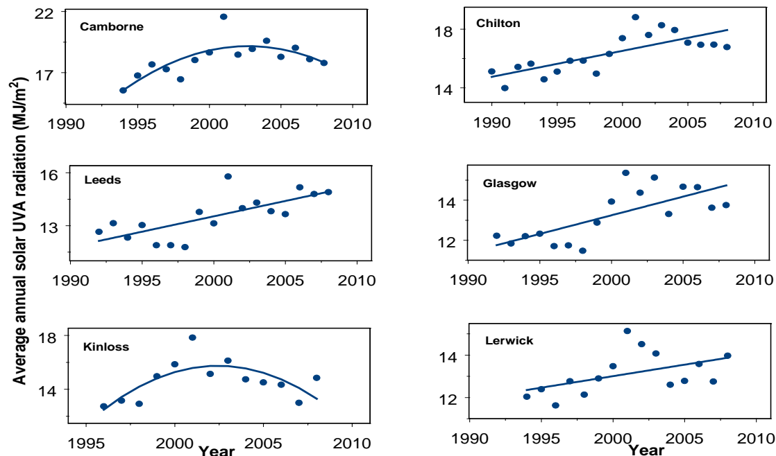
Figure 13: The trend for average annual UVA dose data versus time for the six GB sites: Chilton (1990-2008), Glasgow (1992 – 2008), Leeds (1992 – 2008), Camborne (1994-2008), Lerwick (1994-2008) and Kinloss (1996-2008).
