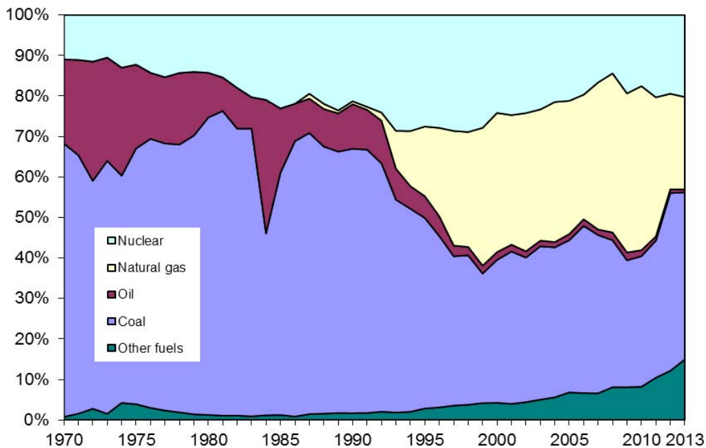
Chart 5.1.1 Percentage shares of fuel input for electricity generation, 1970 to 2013
