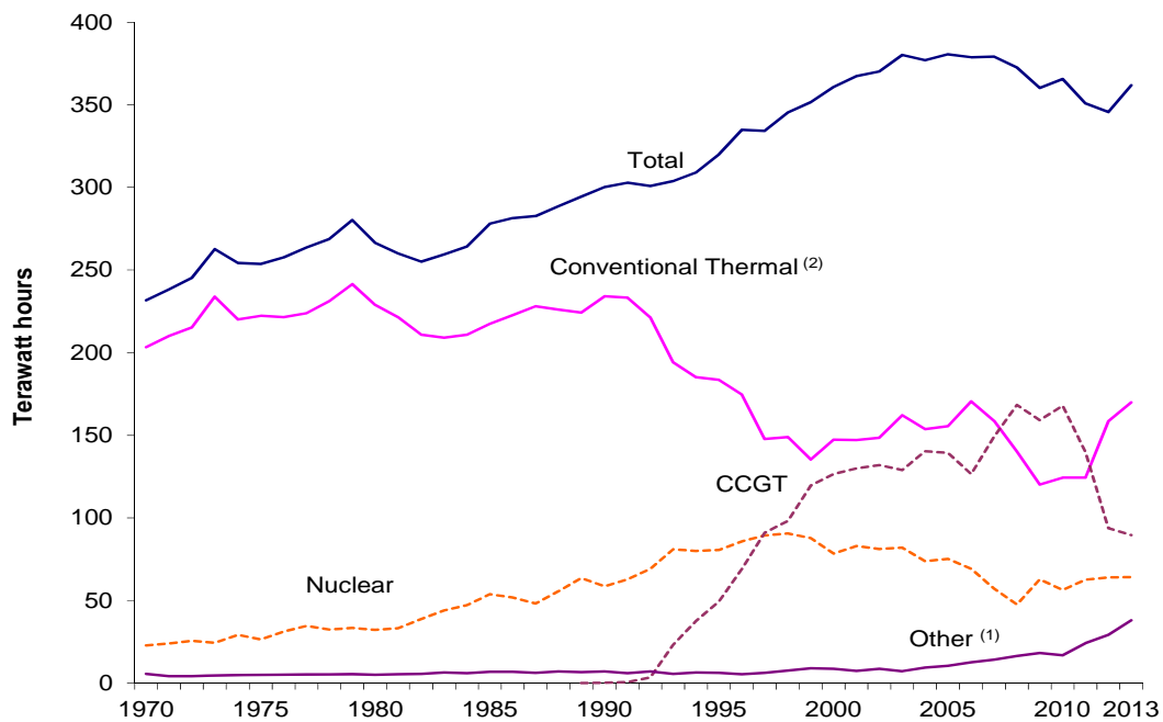
Chart 5.1.2: Gross electricity supplied by all generating companies by type of plant, 1970 to 2013
