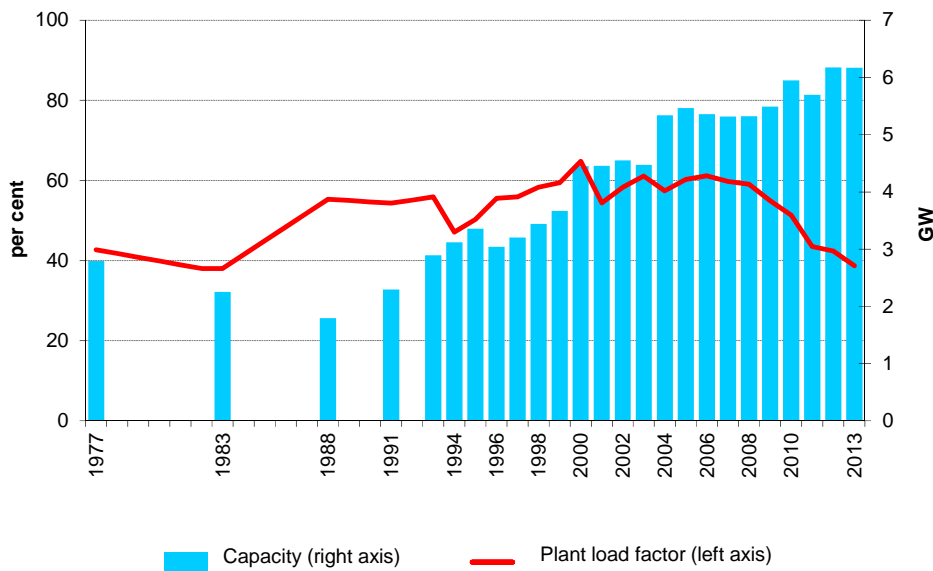
Chart 7.1.1: CHP electricity generation capacity and average load factor 1977 to 2013
