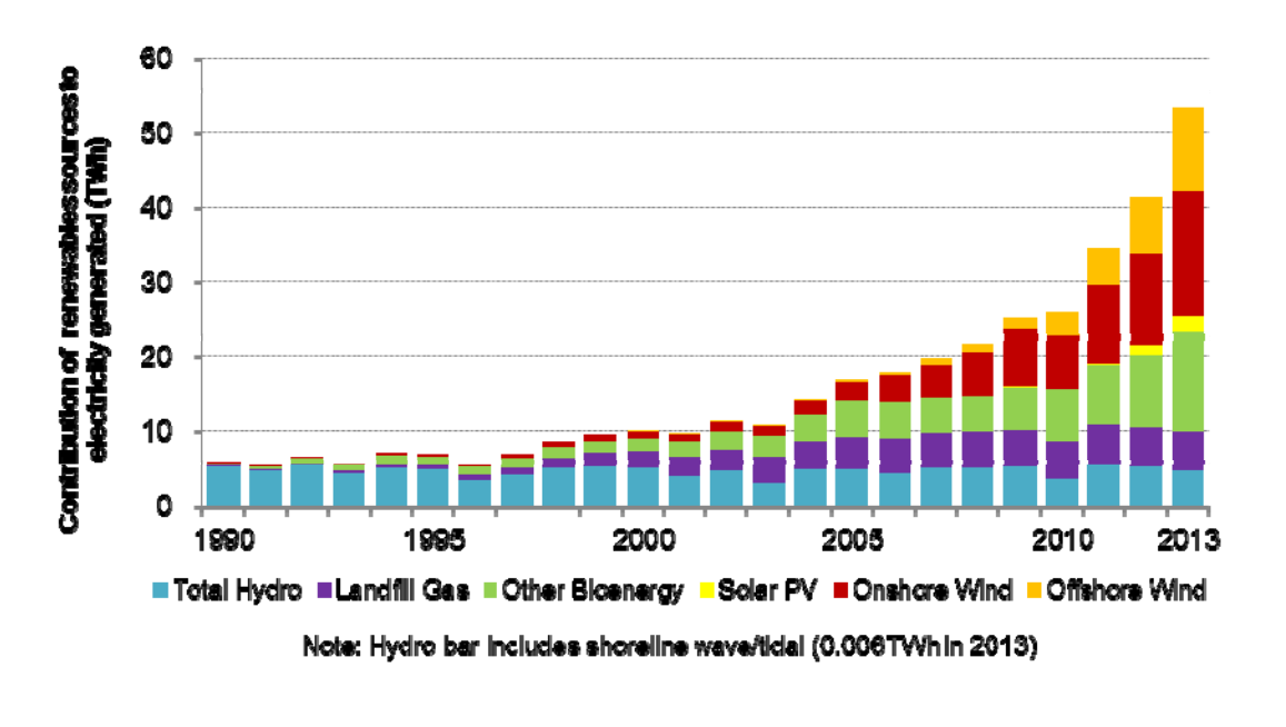
Chart 6.1.2: Electricity generated from renewable sources, 1990 to 2013
