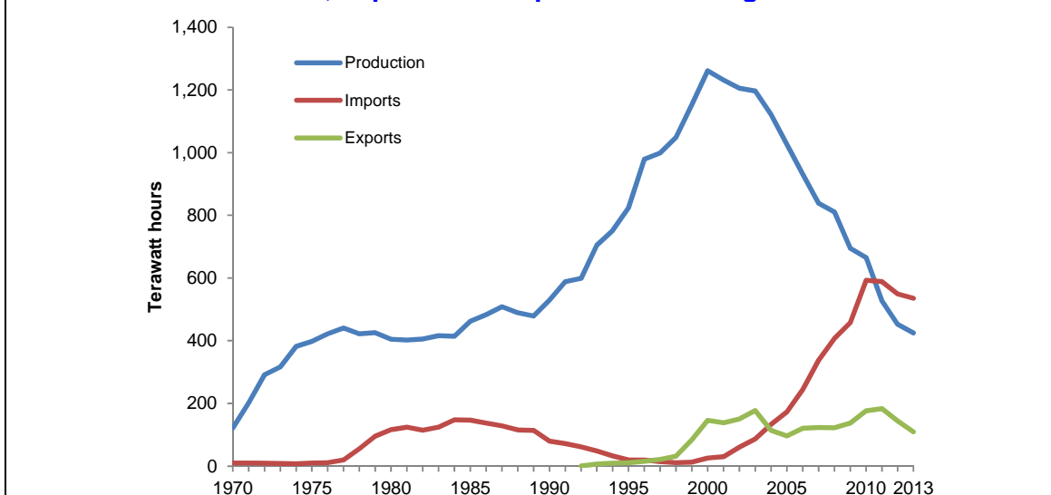
Chart 4.1.1: Production, imports and exports of natural gas 1970 to 2013
