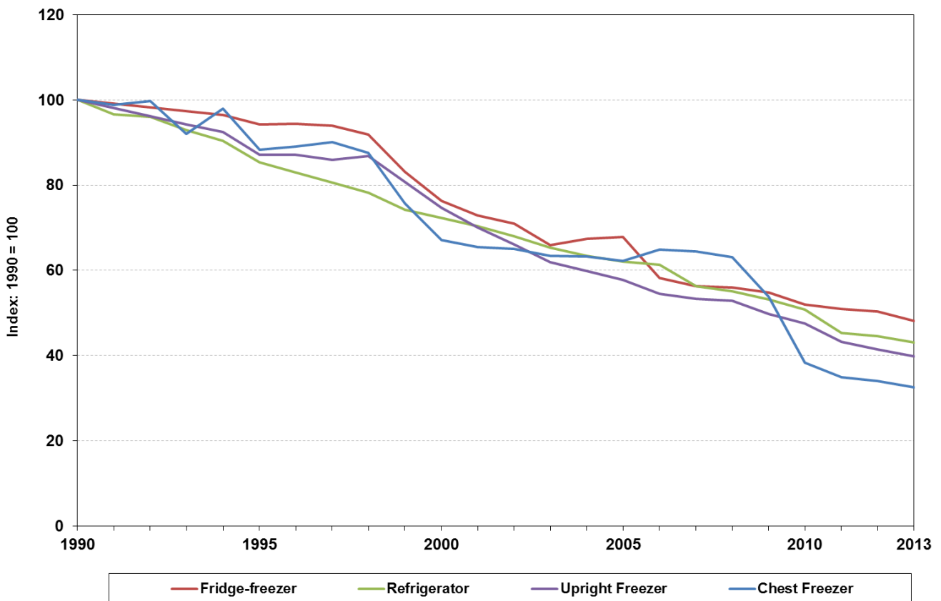
Chart 7 Average energy consumption of new cold appliances, UK (1990 to 2013)
