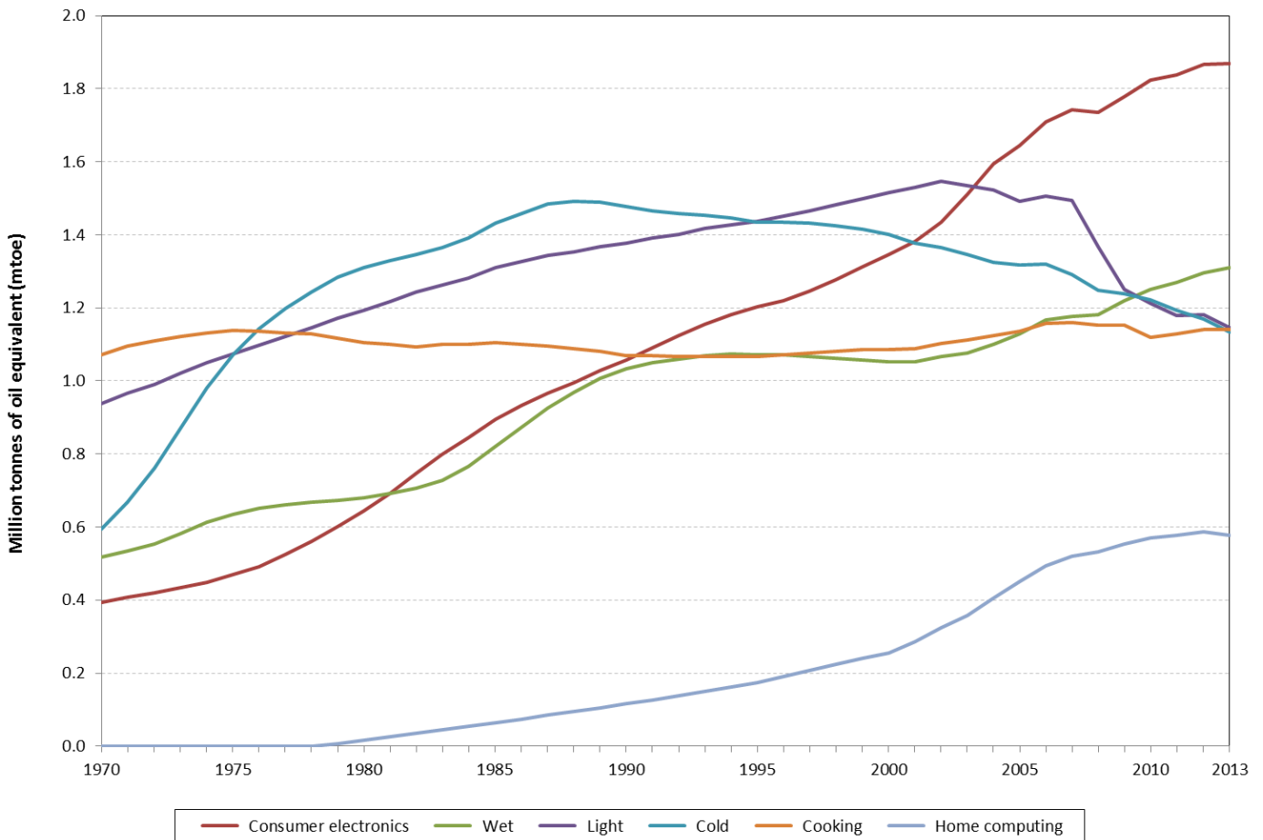
Chart 6 Electricity consumption by household domestic appliance, by broad type, UK (1970 to 2013)
