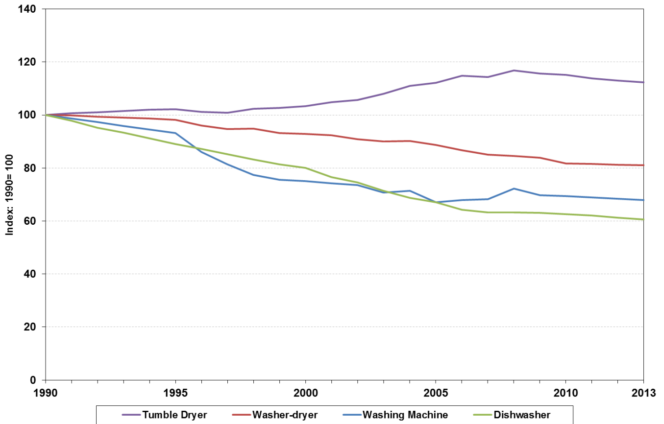
Chart 8 Average energy consumption of new wet appliances, UK (1990 to 2013)
