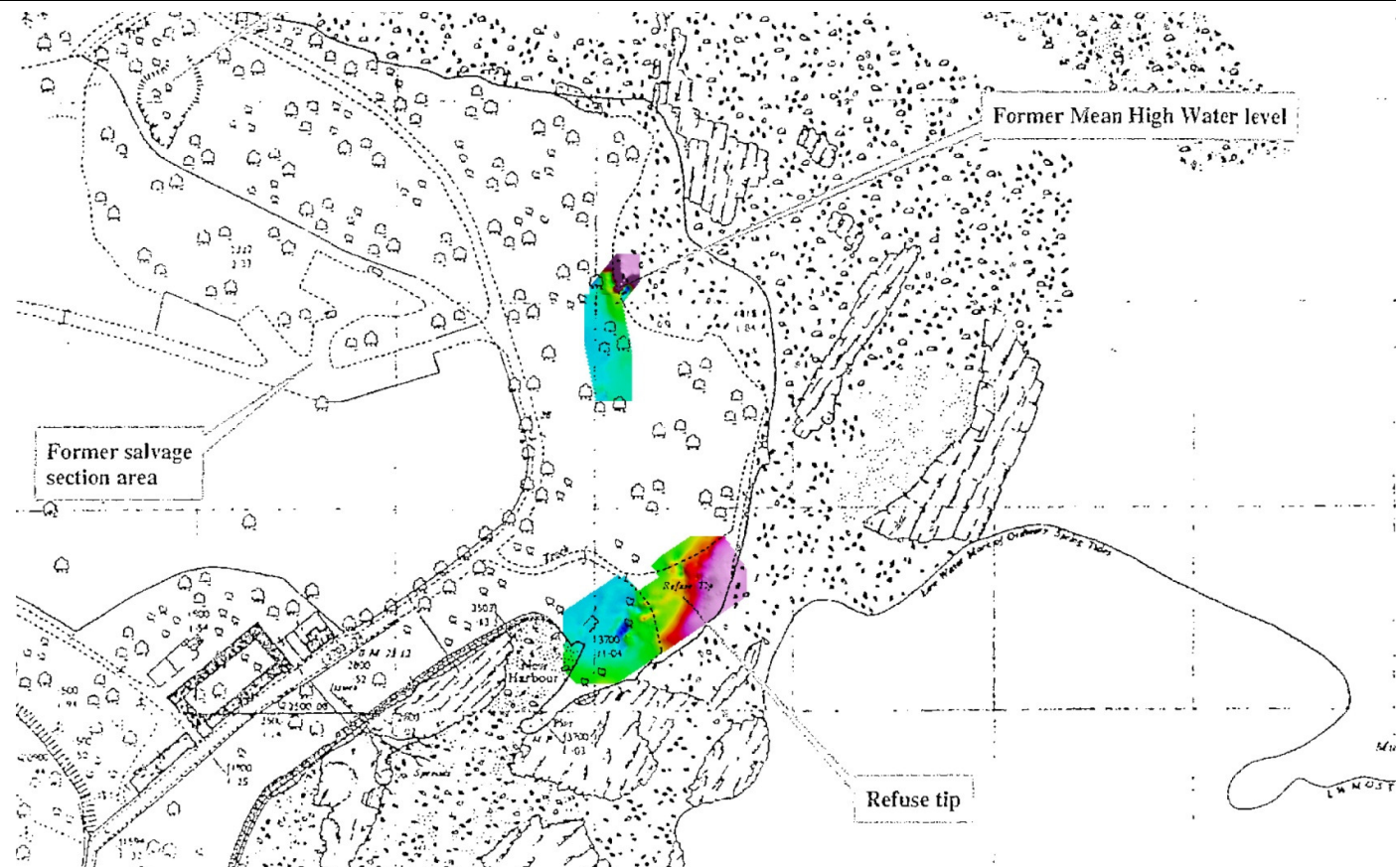
Figure 5: FEM data overlaid on historical mapping
