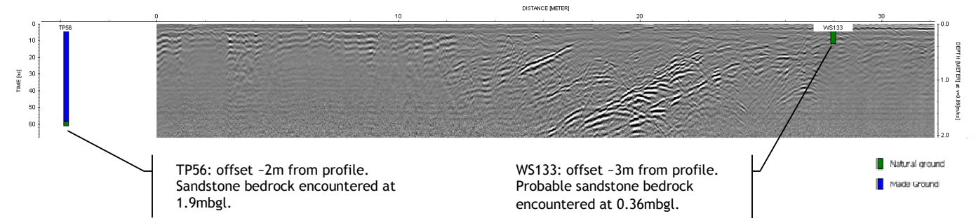
Figure 2: Example radargrams from the south of the Site
