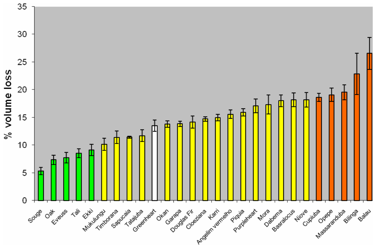
Figure 2: Average volume loss (mean ± Standard Error) after 160,000 cycles for the candidate species compared with Greenheart.
