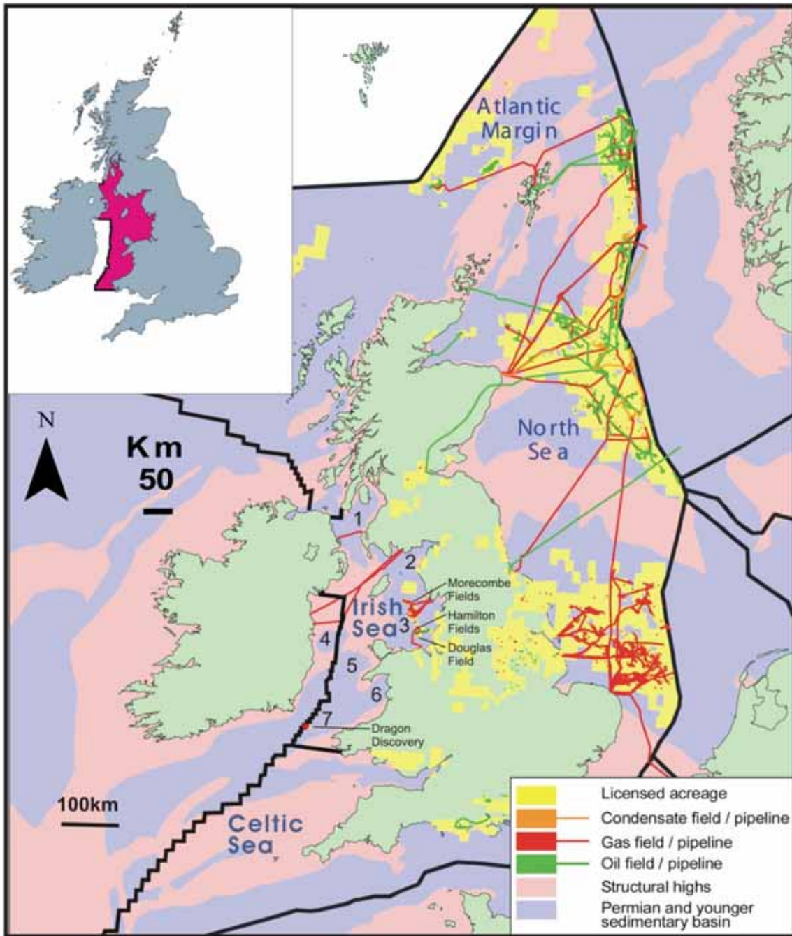
Sedimentary basins: 1 North Channel Basin 2 Solway Basin 3 East Irish Sea Basin 4 Kish Bank Basin 5 Caenarfon Bay Basin 6 Cardigan Bay Basin 7 North Celtic Sea Basin
