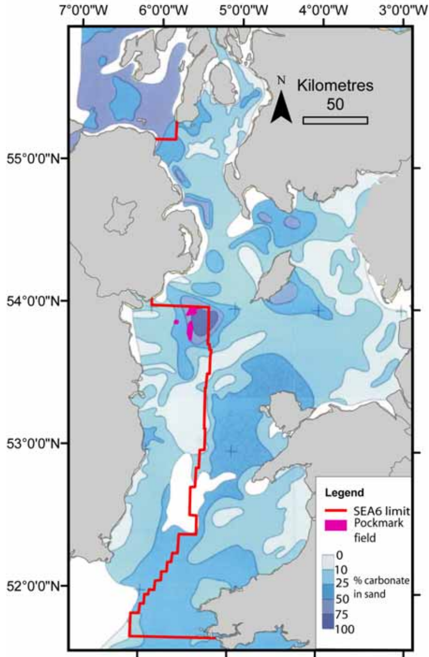
Figure 12 Percentage carbonate in the seabed-sediment sand fraction, and locations of pockmark fields.
