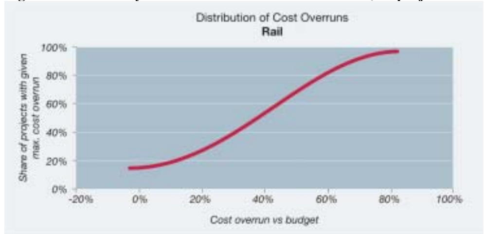
Figure 5 - Probability distribution of cost overrun for rail, 46 projects.
