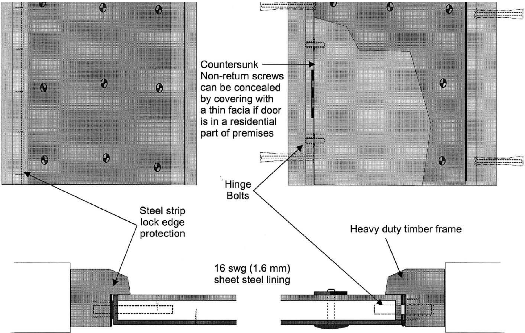
Sectional View
