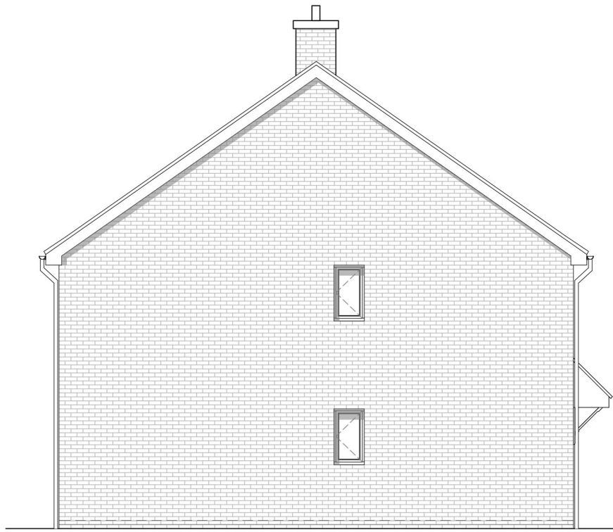
Gable Elevation
