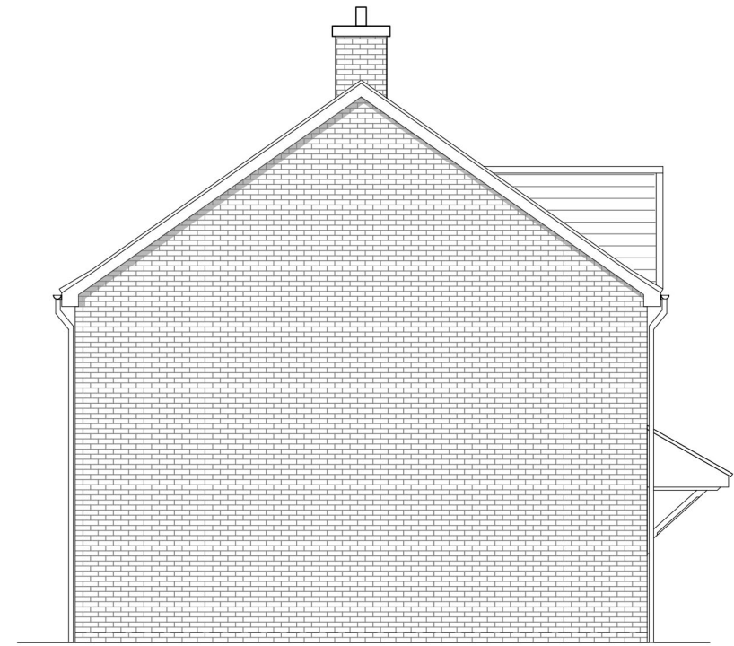
Gable Elevation
