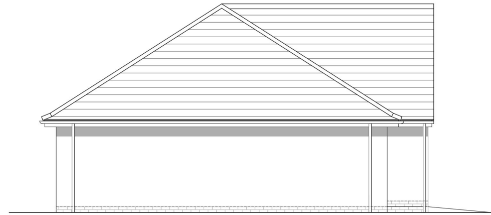
Gable Elevations
