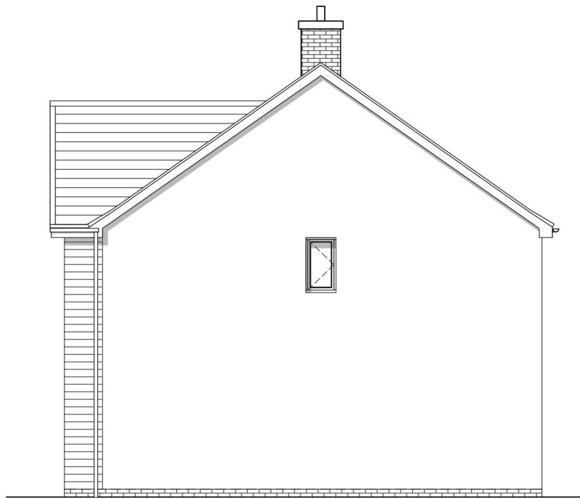
Gable Elevation
