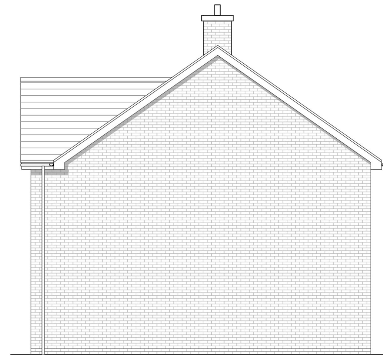
Gable Elevation
