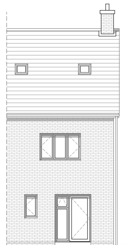
Rear Elevation
