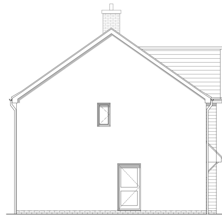
Gable Elevation
