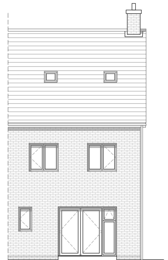
Rear Elevation
