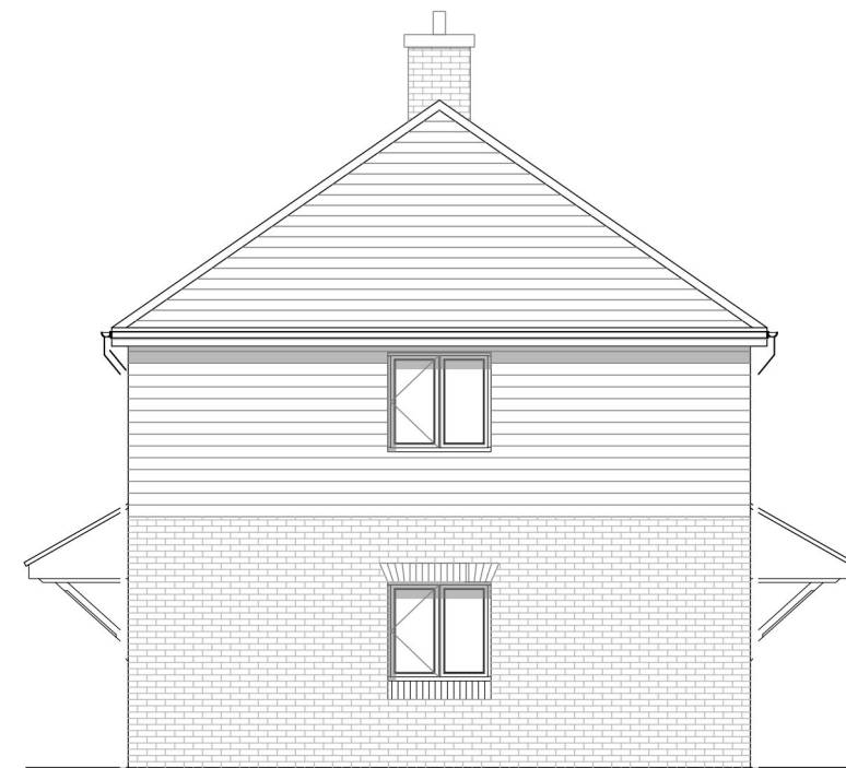
Gable Elevation
