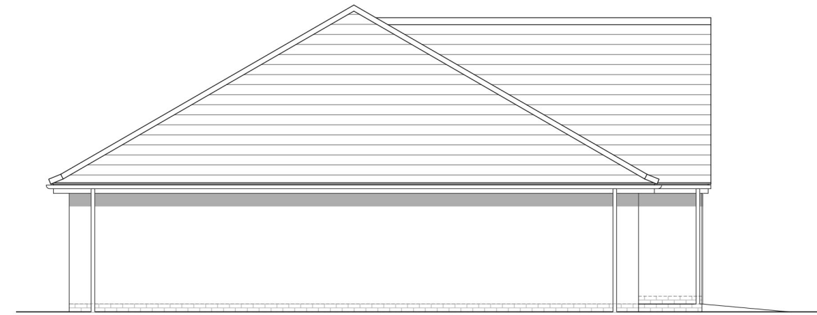
Gable Elevations
