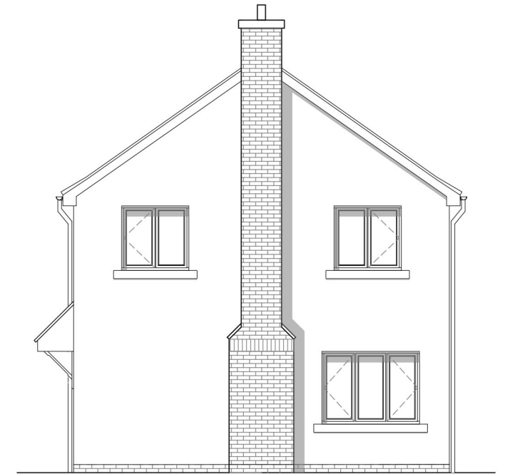
Active Gable Elevation
