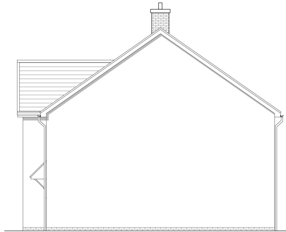
Gable Elevation
