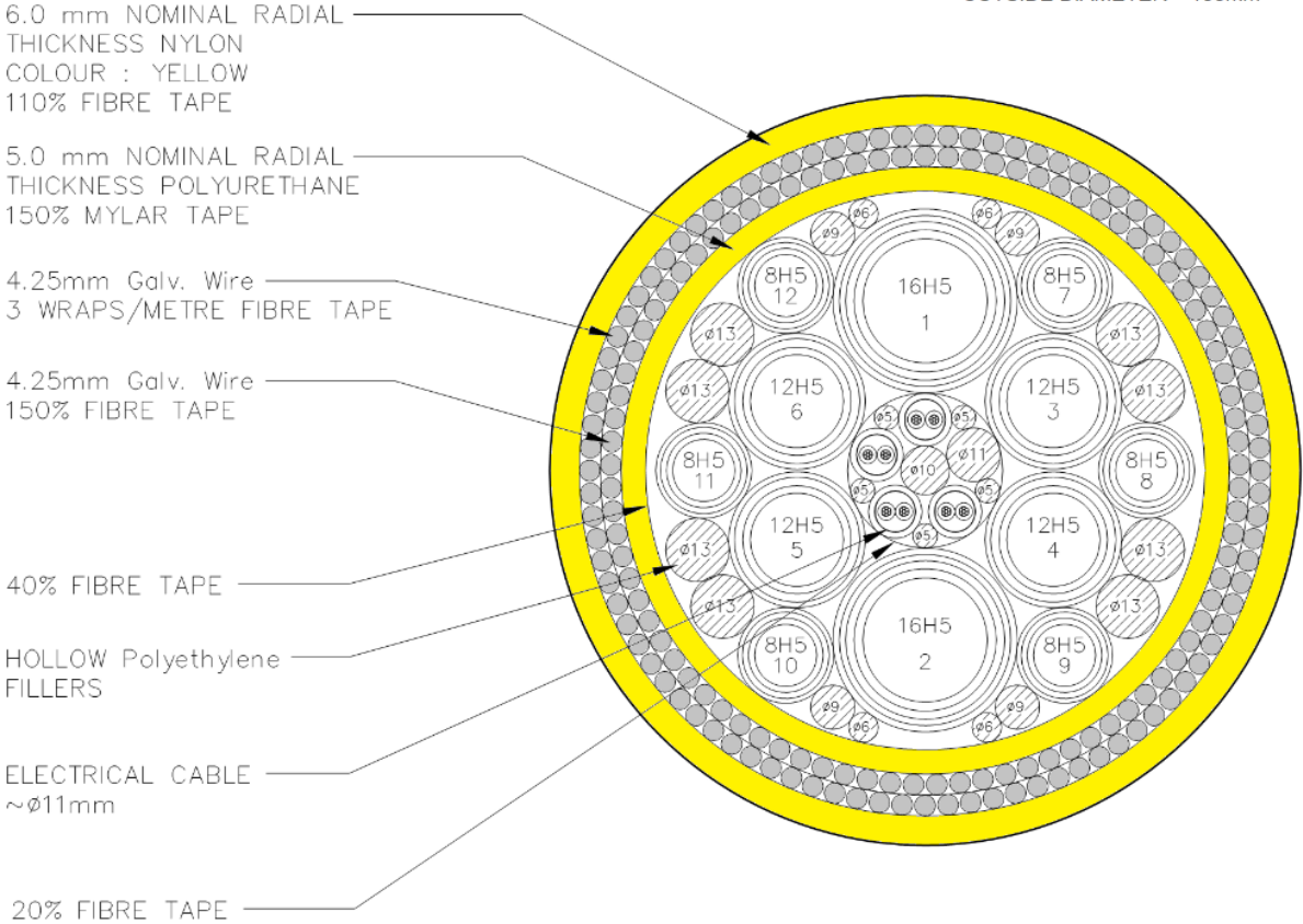
Figure 3.3.1: PLU2544(2) umbilical cross section, 153mm diameter
