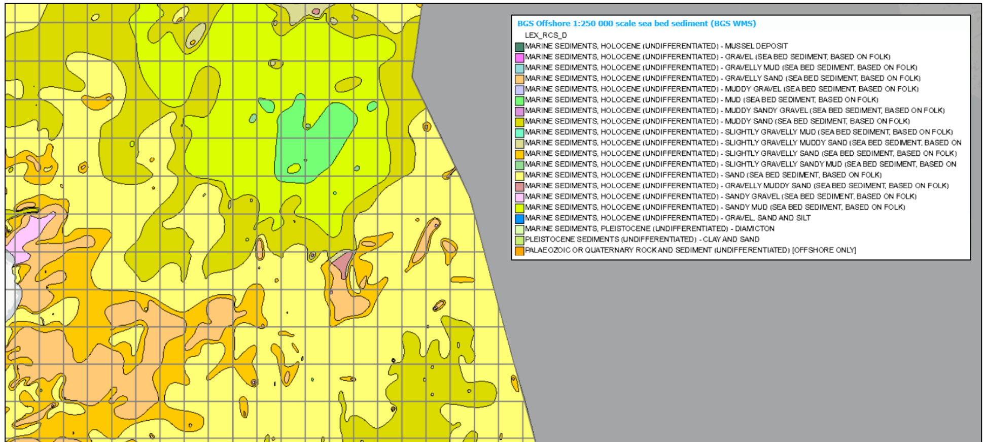
Figure 2.4.2: Sediment Type in Block 22/2
