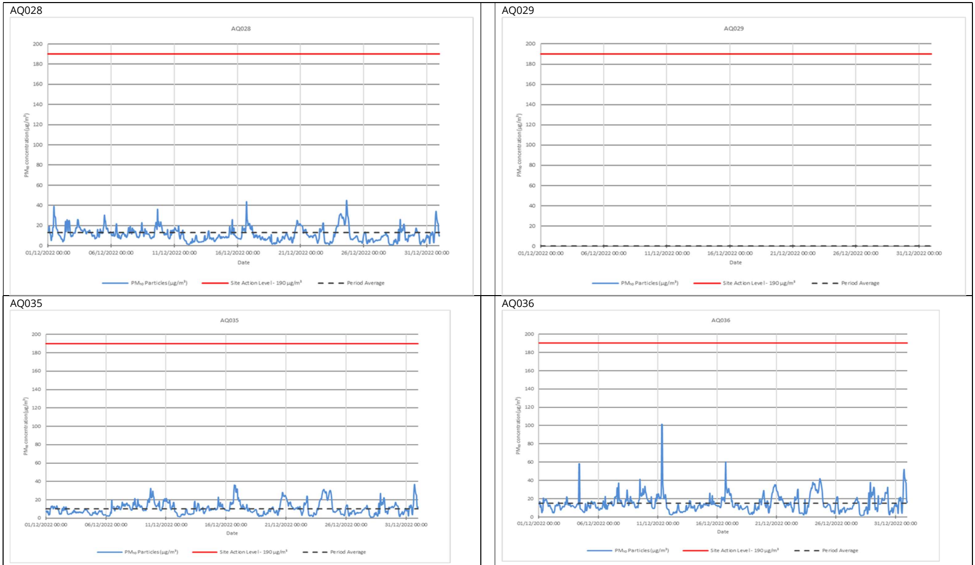
Figure 3: Construction dust 1-hour mean indicative PM 10 concentration for dust monitors
