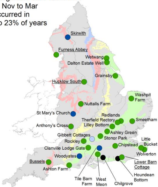
Figure 7.5: Projected groundwater levels at key indicator sites at the end of March 2023. Projections based on four scenarios: 120%, 100%, 80% and 60% of long term average between November 2022 and March 2023. Rainfall statistics based on occurrence in the historic record since 1891. Projections for underlined sites produced by BGS.
