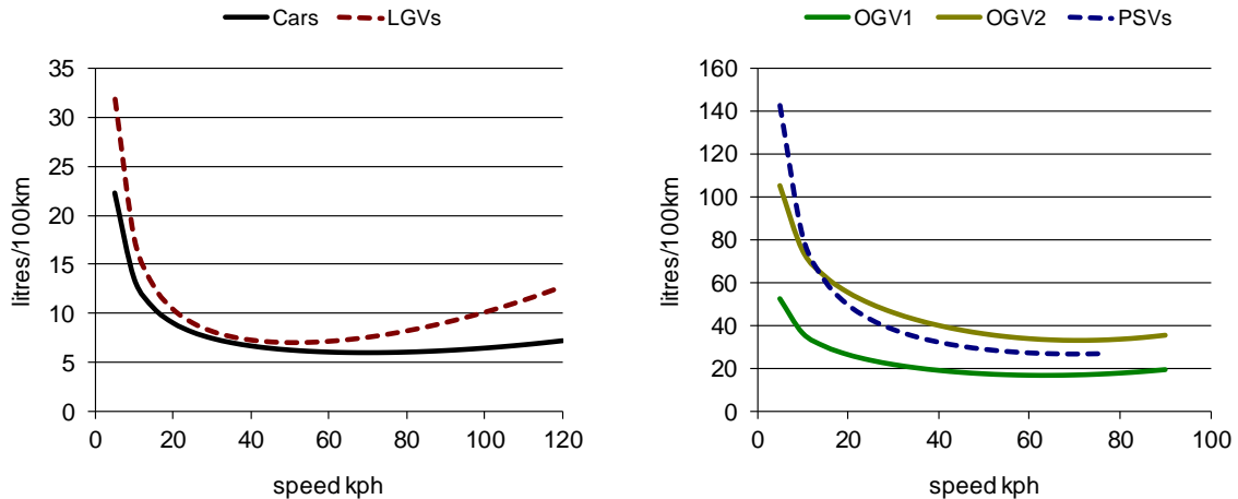
Figure 2 – fuel consumption rates at different speeds (2010 fleet)
