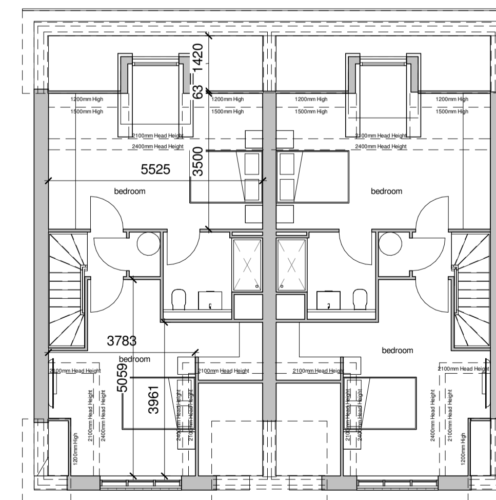
Second floor plan 1 : 100
