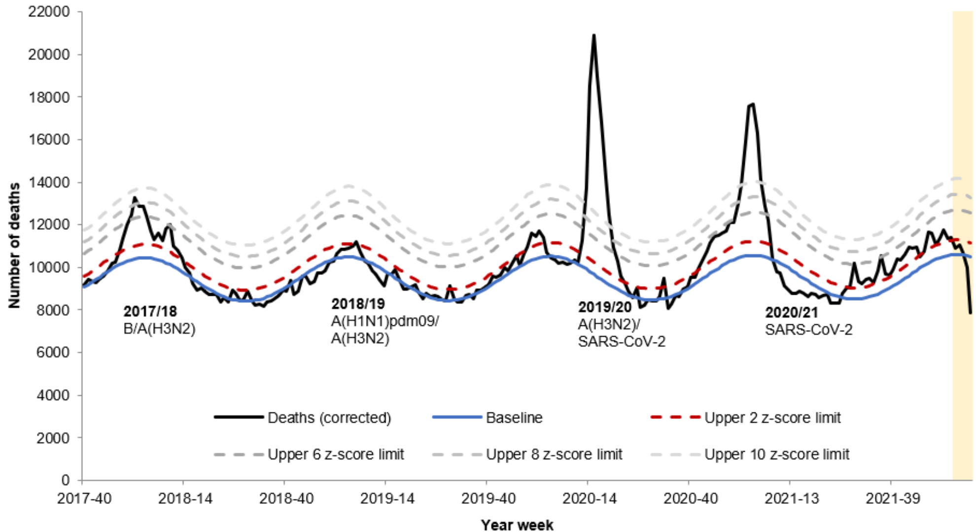
Figure 1: Weekly observed and expected number of all-cause deaths in all ages, with the dominant circulating respiratory virus, England, 2017 to week 7 2022
