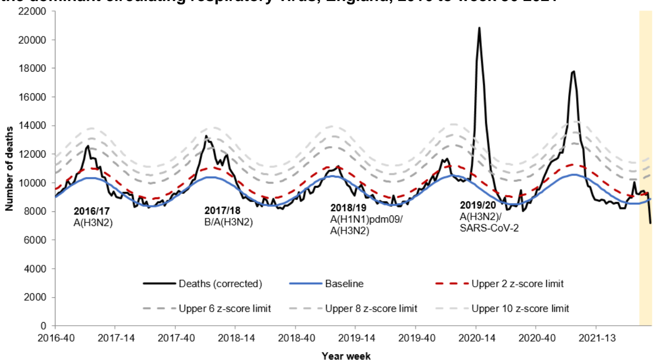
Figure 1: Weekly observed and expected number of all-cause deaths in all ages, with the dominant circulating respiratory virus, England, 2016 to week 36 2021
