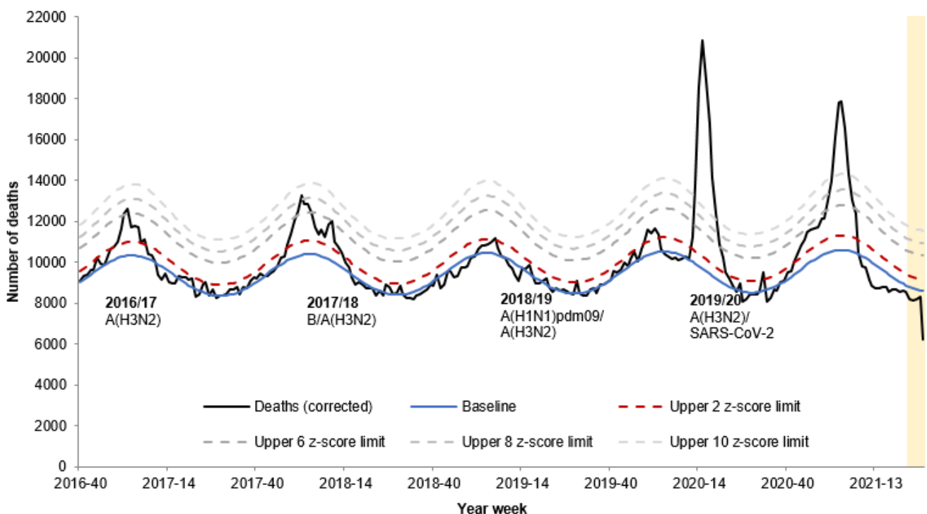
Figure 1: Weekly observed and expected number of all-cause deaths in all ages, with the dominant circulating respiratory virus, England, 2016 to week 27 2021
